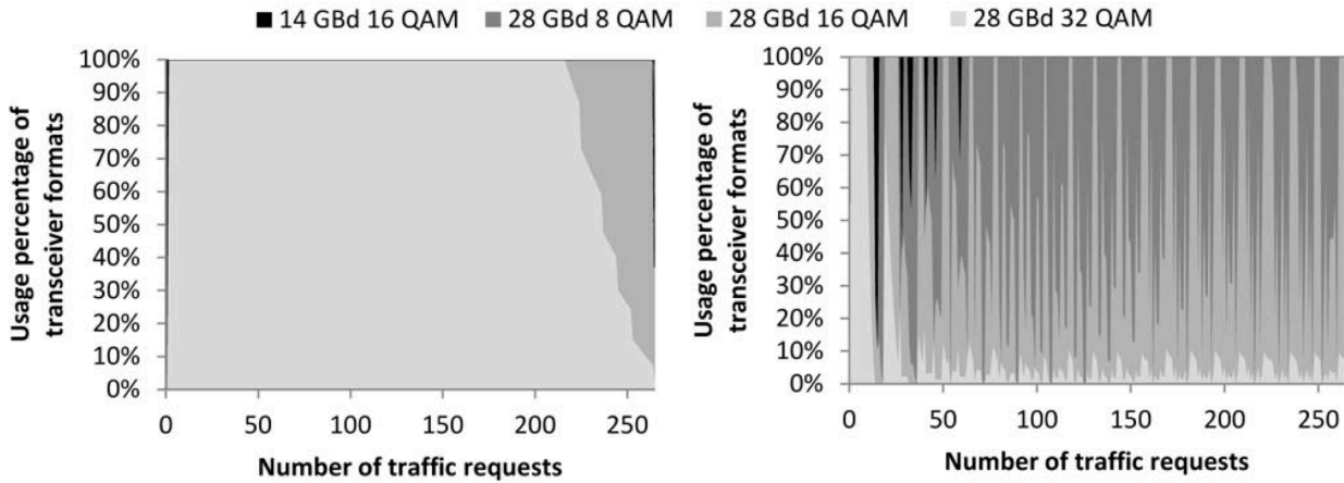
Fig. 6: Modulation formats used when minimizing N_t (left) or H_s (right) for a 100 km fiber with -25 dB attenuation.
