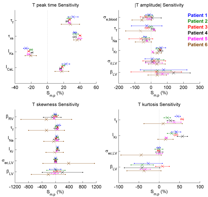
Fig. 7 Significant parameters following sensitivity analysis results for four ECG markers related with the T-wave for the six patients (different colors for each patient): T-wave peak time, T-wave amplitude, T-wave skewness, and T-wave kurtosis. Average values of the 12 ECG lead sensitivities represented by 'x'. Limits of horizontal lines given by the average values \pm the standard deviation in the 12 leads.
