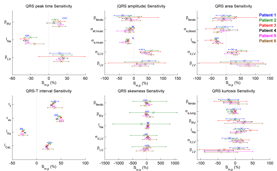
Fig. 6 Significant parameters following sensitivity analysis results for six ECG markers related with the QRS complex for the six patients (different colors for each patient): QRS peak time, QRS amplitude, QRS area, QRS-T interval, QRS skewness, and QRS kurtosis. Average values of the 12 ECG lead sensitivities represented by 'x'. Limits of horizontal lines given by the average values \pm the standard deviation in the 12 leads.
