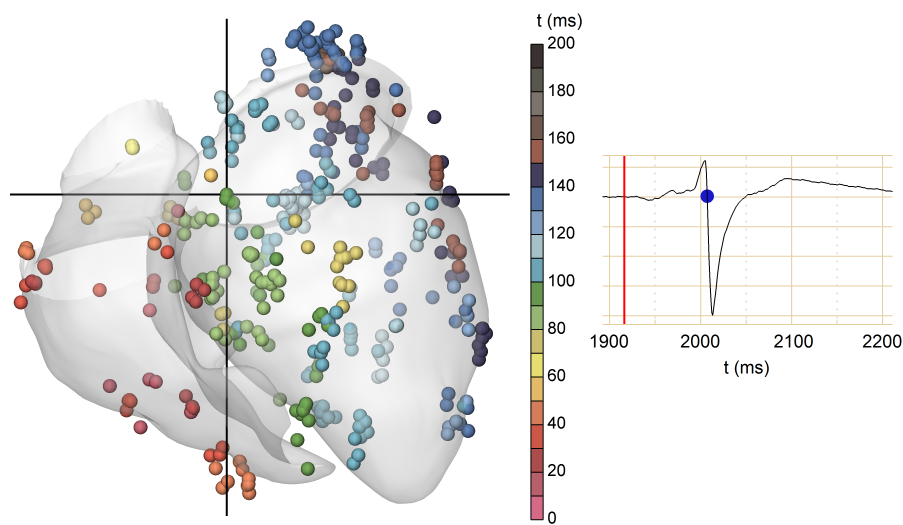
Fig. 1 Modeled endocardial surfaces of RV and LV for patient 5 and measured activation times at NOGA recording sites in a color scale (left panel). Example of an electrogram recorded at the LV endocardium at the position of the crosshair in the left panel (right panel), together with the time of QRS onset (vertical red line) and the activation time (blue dot).
