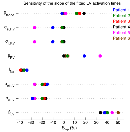
Fig. 5 Significant parameters following sensitivity analysis results for the slope of the fitted line between simulated and measured activation times for the six patients (different colors for each patient).
