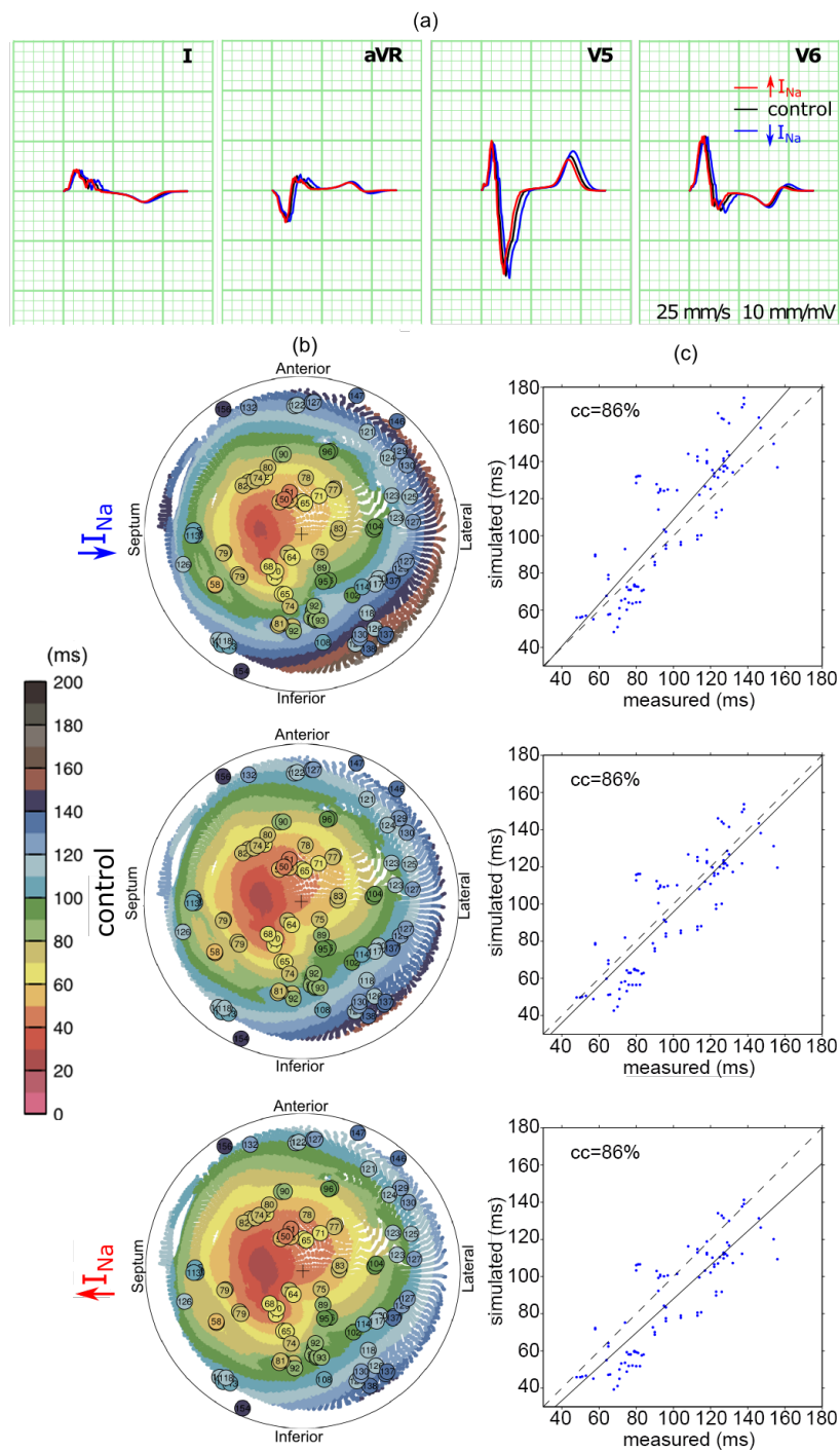
Fig. 4 Simulation results. (a) ECG for patient 2. Leads I, aVR, V5, and V6 with I_{Na} reduction by 30% (blue), no changes (black), and I_{Na} increase by 30% (red). (b) Polar diagram of the LV endocardium showing measured activation times (circles with time in milliseconds) and simulated activation times (colored dots). Apex is marked with a cross, '+', at the center of the diagram. (c) Simulated versus measured activation times on the LV endocardium. Correlation coefficients are shown.
