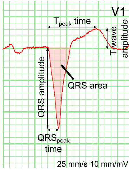
Fig. 3 Example of lead V1 of a clinically measured ECG with five of the markers included in the sensitivity analysis: QRS peak time, QRS amplitude, QRS area, T peak time and T-wave amplitude.
