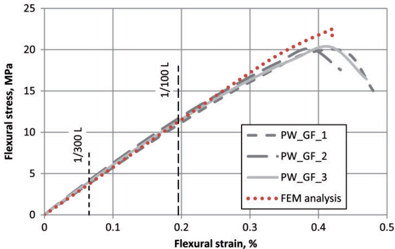
Figure 17. Flexural stress/strain curves for PW_GF sandwich panels.
