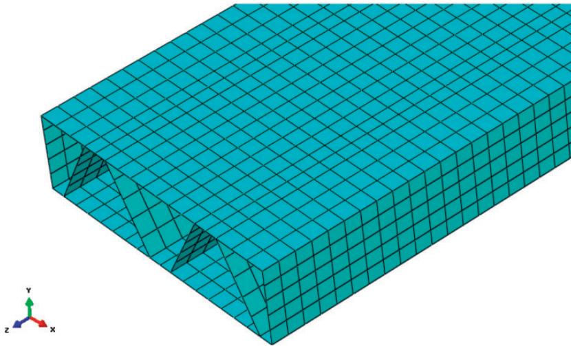
Figure 10. Finite element model of PW_GF sandwich panel.
