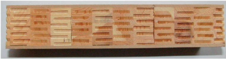
Figure 2. Section of the sandwich panel with HDF surface and cellular wood core (CW_L).
