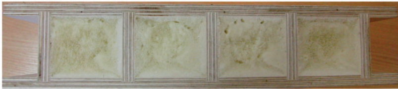
Figure 3. Plywood sandwich panel vertical stiffener and foam core (PW_F).
