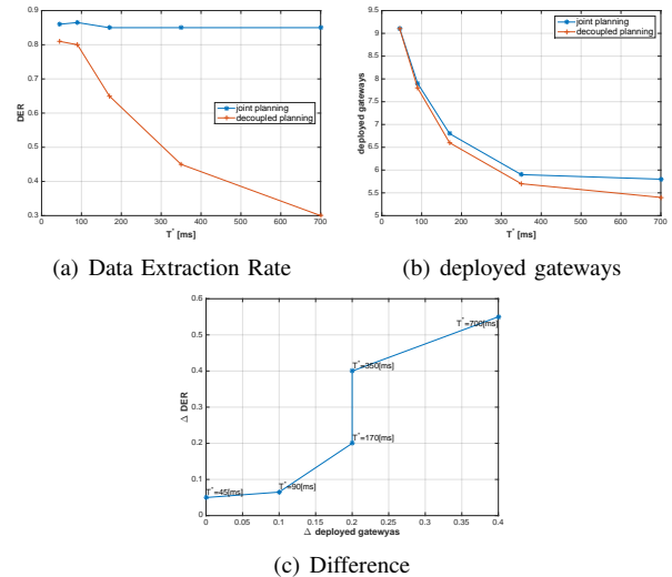
Fig. 5. Difference of number of deployed gateway and data extraction rate when joint and decoupled planning are used. M = 16 .
