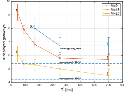
Fig. 2. Number of deployed LoRaWAN gateways versus target values for end-to-end latency for different numbers of available candidate sites ( M ). N = 200 . \gamma = 0.8
