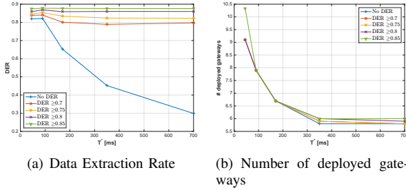
Fig. 4. Data extraction rate and number of deployed gateways for different target maximum transmission delay and different minimum required data extraction rate values. M = 16 .
