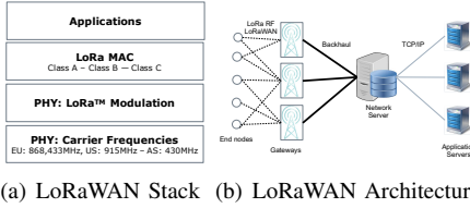
Fig. 1. LoraWAN communication protocol stack (a) and LoraWAN network architecture and components (b).
