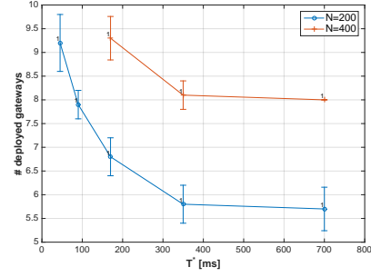
Fig. 3. Number of deployed LoRaWAN gateways versus target values for end-to-end latency for different numbers end devices ( N ). M = 16 .
