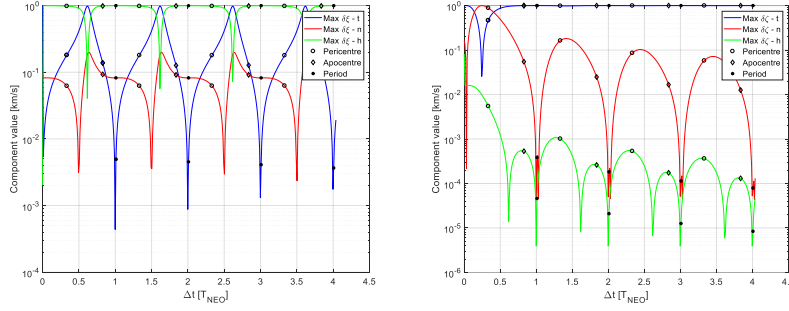
Fig. 3.3 Components of the maximum \delta\xi\zeta (left) and \delta\zeta\zeta (right) deviation direction for 2010 RF 12
