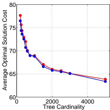
Fig. 1. Average cost of optimal solution as a function of tree cardinality with actuation limits A_1 , \Omega_1 (blue line), and A_2 , \Omega_2 (red line).
