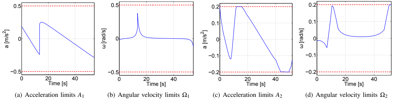
Fig. 3. Actuation profiles of the optimal solutions obtained with N = 1000 (solid blue) and corresponding actuation limits (dashed red).
