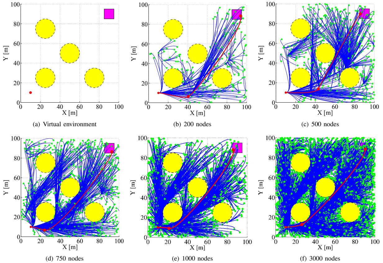
Fig. 2. A planning experiment: start pose (red dot), goal area (magenta square), obstacles (yellow circles), tree nodes (green crosses), tree edges (solid blue), optimal solution (solid red), optimal trajectory nodes (red circles).
