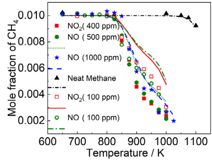
Fig. 2. Mole fractions of methane with various additions of \text{NO}_2 (400 and 100 ppm) and \text{NO} (1000, 500 and 100 ppm) under stoichiometric condition.
