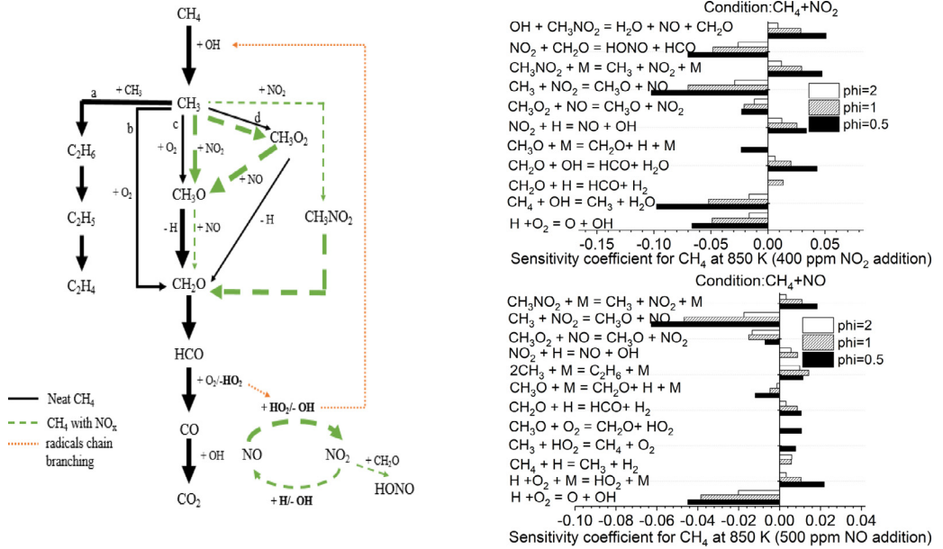
Fig. 4. Left: Reaction path diagram for CH 4 oxidation in presence of NO x (Φ = 1, T = 850 K). Solid lines represent the main reaction routes occurring during the oxidation of neat CH 4 (1100 K); dashed lines highlight the main changes due to the presence of NO x . The size of the arrow is proportional to the flow rate of the given reactions. Right: CH 4 sensitivity coefficient at 850 K in the presence of NO 2 (upper: 400 ppm) and NO (bottom: 500 ppm).
