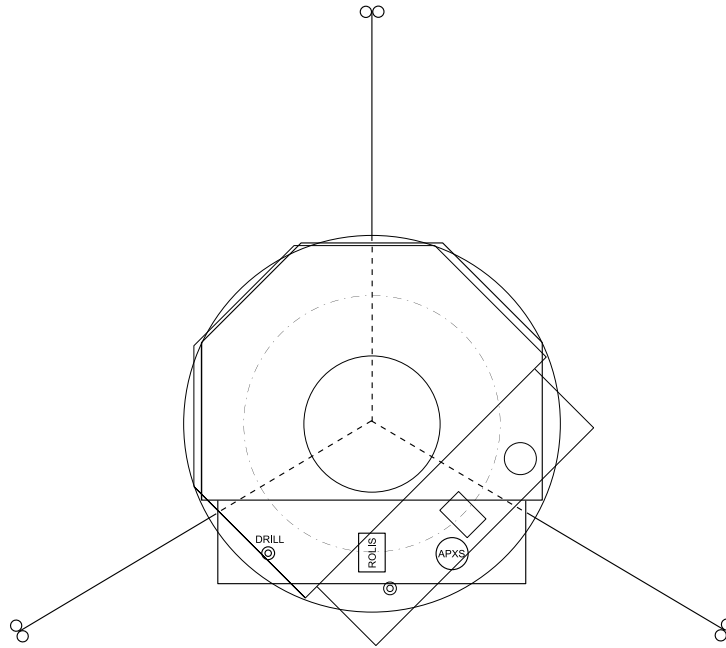
Figure 12: ROLIS, drill, and APXS accommodation on the Philae instrument deck.
