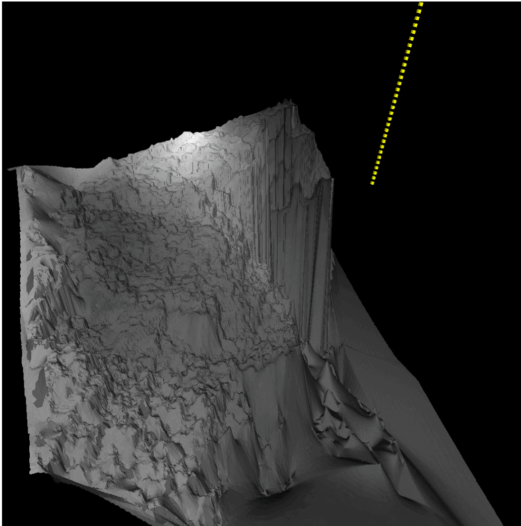
Figure 14: Drilling trajectory (yellow dots) and 3D local model of the comet surface.
