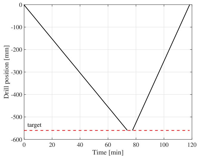
Figure 9: Drill position profiles during the roto-translation to 560 mm and the translation back to 0 mm.
