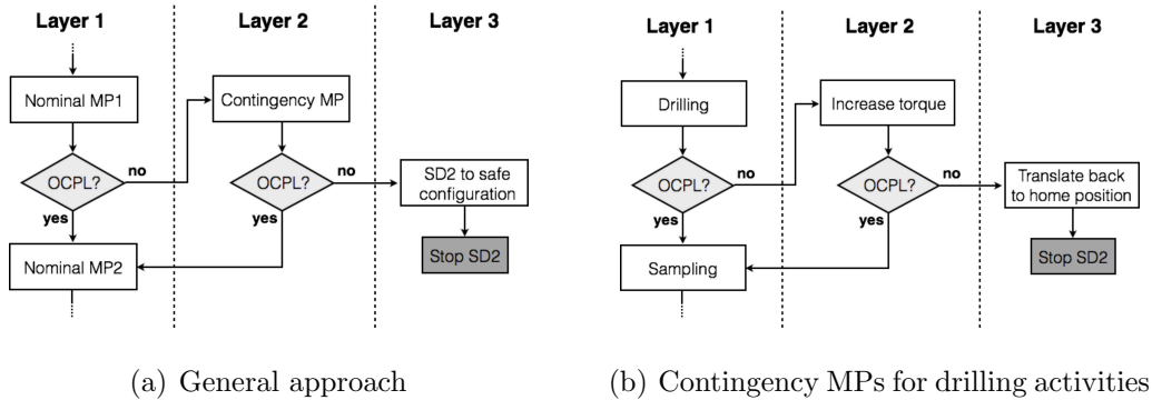
Figure 7: Management of SD2 emergencies by CDMS.
