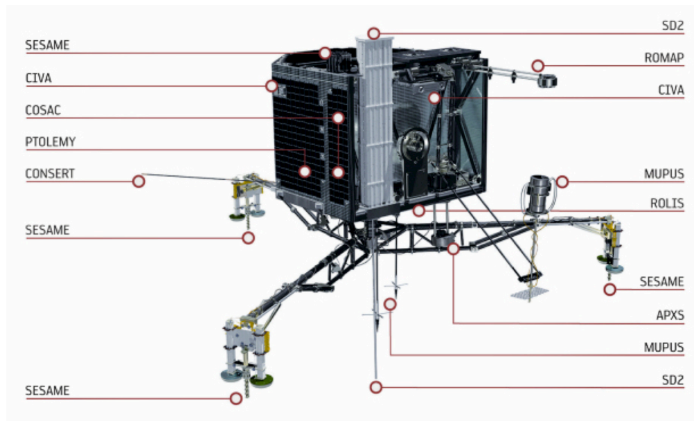
Figure 1: The lander Philae onboard Rosetta mission (Credits: ESA/ATG medialab).
