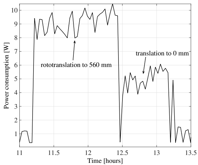
Figure 10: SD2 power consumption during the roto-translation to 560 mm and the translation back to 0 mm.
