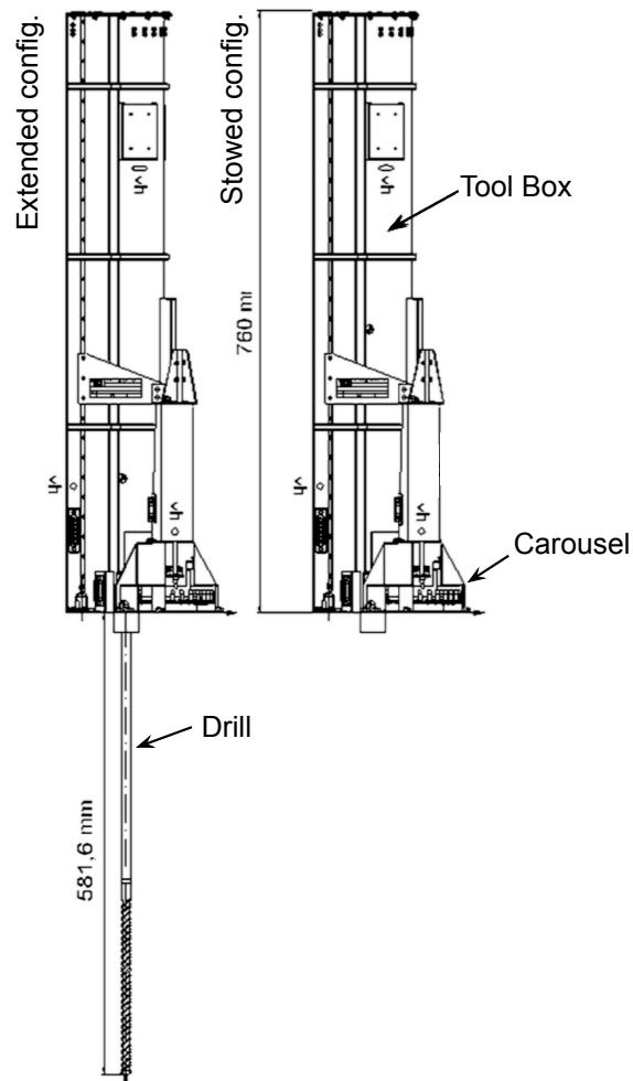
Figure 2: SD2 mechanical unit in stowed and extended configuration (Credits: Selex-ES.
