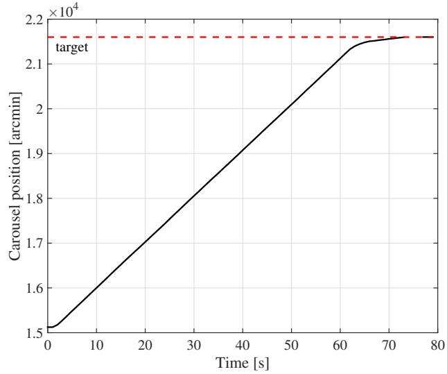
Figure 11: Carousel position profile during the Carousel rotation back to home position for PTOLEMY sniffing activities.
