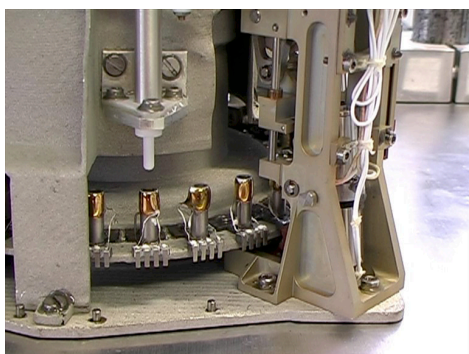
(a) High-temperature ovens
