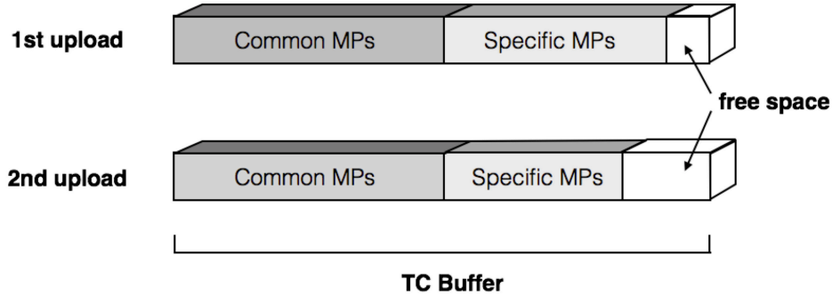
Figure 6: TC buffer allocation strategy.
