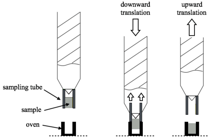
Figure 5: Schematic representation of the sample release operation.
