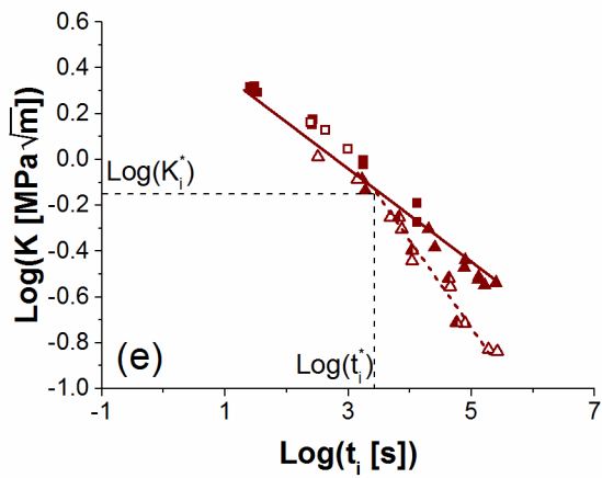
Figure 6 - Crack initiation behaviour of HDPE-MONO at different temperatures: (a) 23°C, (b) 31°C, (c) 40°C, (d) 50°C, (e) 60°C. The ductile to brittle transition and the effect of the two environments can be observed in (a) and (c,d,e) respectively.
