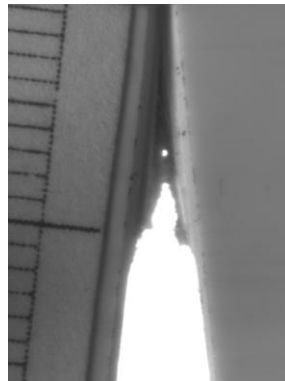
Figure 2 – Example of a video frame recorded during a fracture test. The formation and evolution of the rim film prevents visual determination of crack length with sufficient accuracy.
