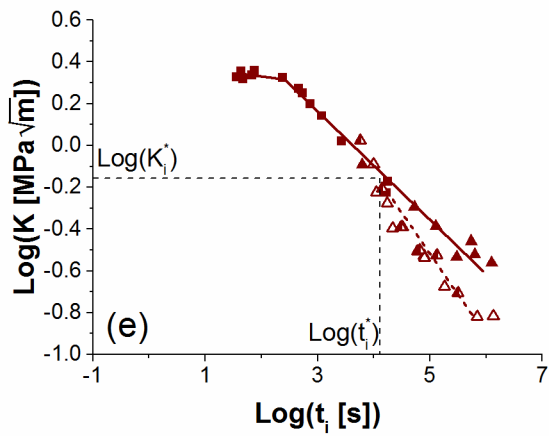
Figure 5 - Crack initiation behaviour of HDPE-BI at different temperatures: (a) 23°C, (b) 31°C, (c) 40°C, (d) 50°C, (e) 60°C. The ductile to brittle transition and the effect of the two environments can be observed in (a,c,e) and (c,d,e) respectively.
