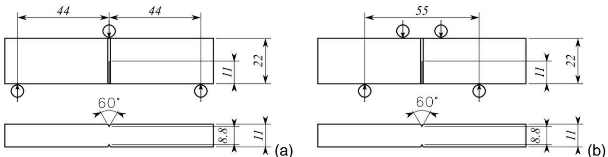
Figure 1 - Specimen geometries and nominal dimensions (in mm). (a) SENB in three point bending for constant displacement rate tests; (b) SENB in four point bending configuration for constant load (creep) tests.
