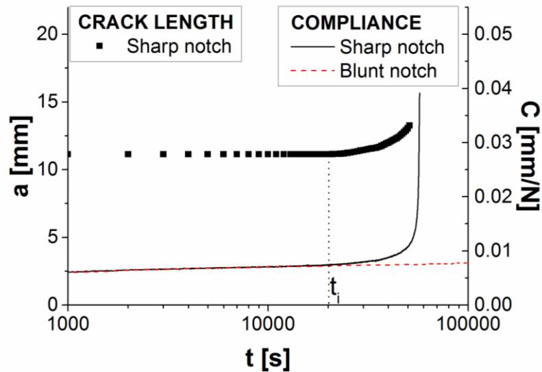
Figure 3 - Sample compliance-time curves for HDPE-MONO at 60°C and an initial applied stress intensity factor of 0.5 \text{ MPa}\cdot\text{m}^{1/2} . Crack length can be determined by comparing the compliance of blunt and sharp notched samples as reported in [17].
