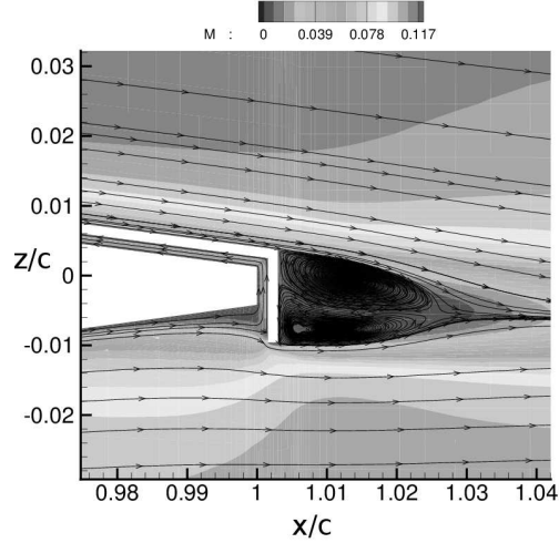
Figure 2: Mach number flow field and streamlines close to the trailing edge of the L-tab equipped blade section, resulting from CFD simulations; angle of attack = 0 deg., freestream Mach number M = 0.117 , Reynolds number Re = 1 \cdot 10^6 .
