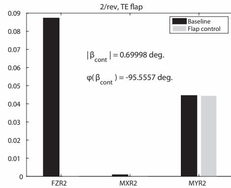
(b) 2/rev, control with the TE flap
