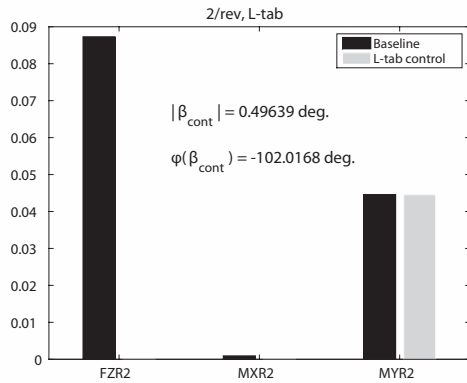
(a) 2/rev, control with the L-tab
