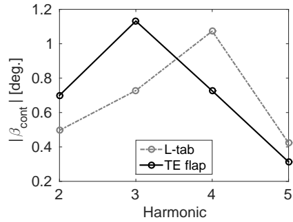
Figure 9: Amplitude of the HHC computed control inputs versus the minimized harmonic. The results attained for both the L-tab and the TE flap are reported.
