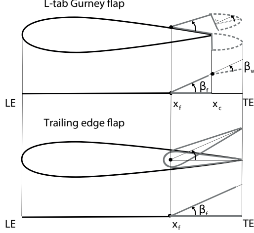
Figure 3: Thin line geometry for the ROMs; L-tab Gurney flap with the CRV (top) and classical plain trailing edge flap (bottom).
