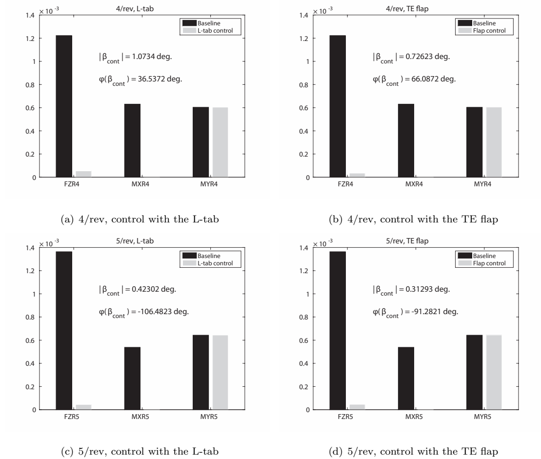
Figure 8: Rotating frame blade root 4/rev and 5/rev harmonic components of vertical force (FZ), bending (MX) and pitching (MY) moments with and without the addition of the movable device, controlled with the HHC approach; \mu = 0.2 .
