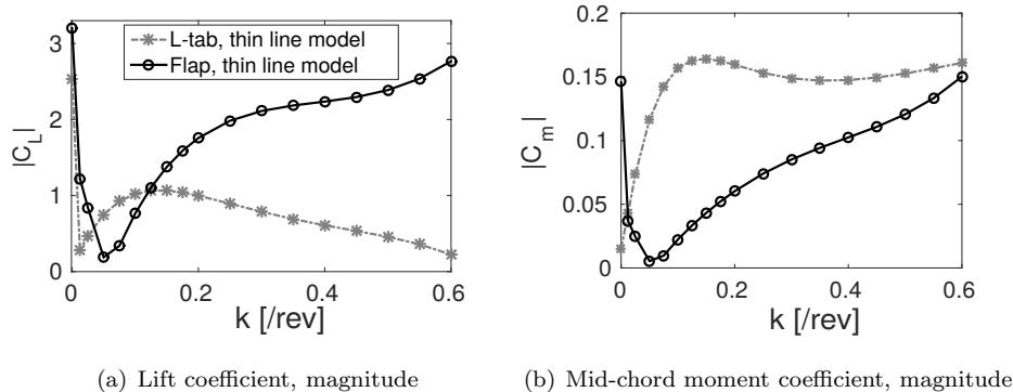
Figure 4: Magnitude of the lift and pitching moment coefficients vs. the reduced frequency. Comparison between the L-tab and the flap models at \beta = 1 deg. and \beta = \sin(\omega t) deg.; M = 0.117 , Re = 1 \cdot 10^6 .
