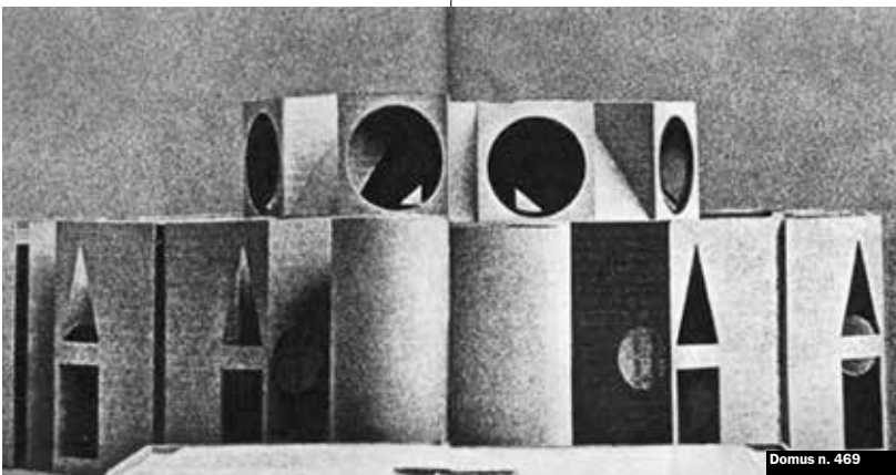
1968 Modello del National Assembly Building di Dacca, Pakistan, progetto di Louis Kahn/ Louis Kahn's design for the National Assembly Building in Dhaka, Pakistan
