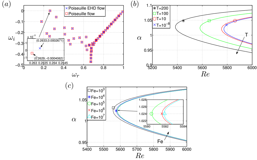
FIGURE 8. (a) Comparison of two spectra for T = 10^{-8} and T = 200 at C = 100 , Re = 5600 , Fe = 10^5 , \alpha = 1 , \beta = 0 . (b) Effect of T on the neutral stability curve with cross-flow at C = 100 , Fe = 10^5 , M = \sqrt{T/M^2} , \beta = 0 . The direction of the arrow indicates increasing T . (c) Effect of Fe on the neutral stability curve with cross-flow at C = 100 , T = 100 , M = \sqrt{T/M^2} , \beta = 0 . The direction of the arrow indicates increasing Fe .
