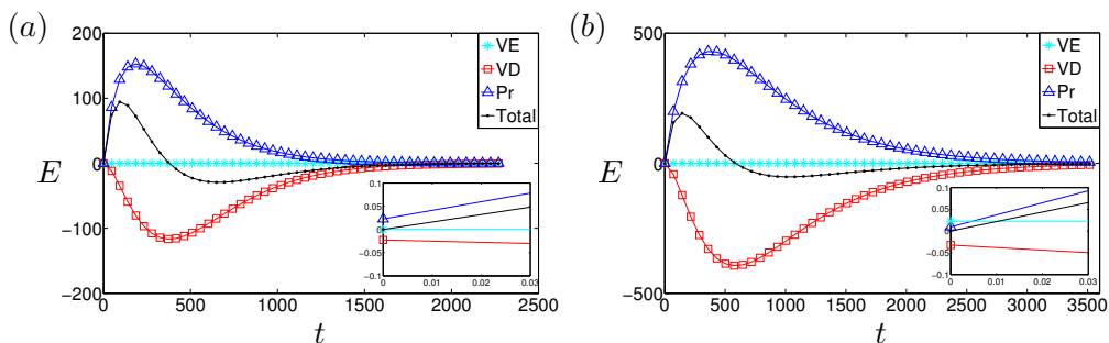
FIGURE 11. Energy analysis over a finite time horizon at C = 100 , Re = 5000 , Fe = 10^5 , \alpha = 0 . (a) T = 10^{-8} , \beta = 2.05 ; (b) T = 100 , \beta = 2.36 .
