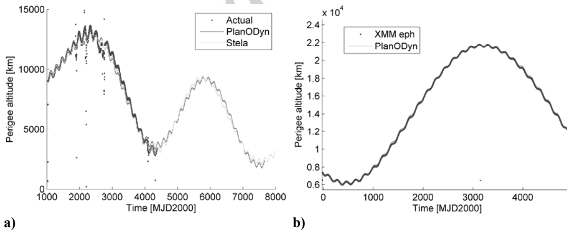
Figure 3. HEO perigee altitude evolution. Blue: actual ephemerides, Red: propagation with PlanODyn , cyan: propagation with STELA software 20 . A) INTEGRAL and b) XMM-Newton.
