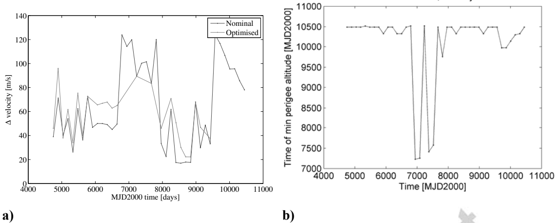
Figure 4. Required \Delta v to de-orbit INTEGRAL. The blue line refers to the nominal solutions from the global optimisation, the red lines to the optimised solutions.
