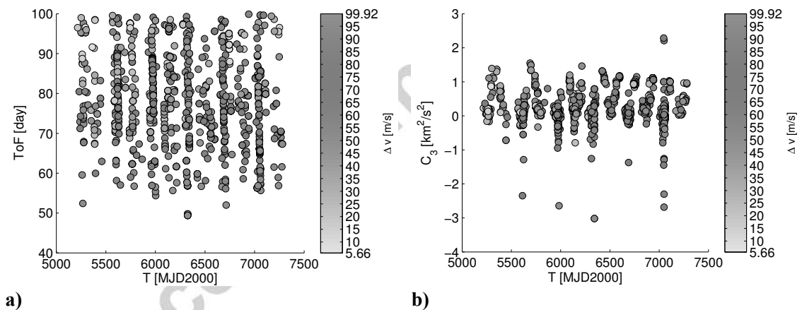
Figure 11. A) Time of flight and b) C_3 value to impact the Moon as a function of the time of departure from the Gaia LPO in MJD2000. Solutions are colour-coded according to the \Delta v cost in m/s.
