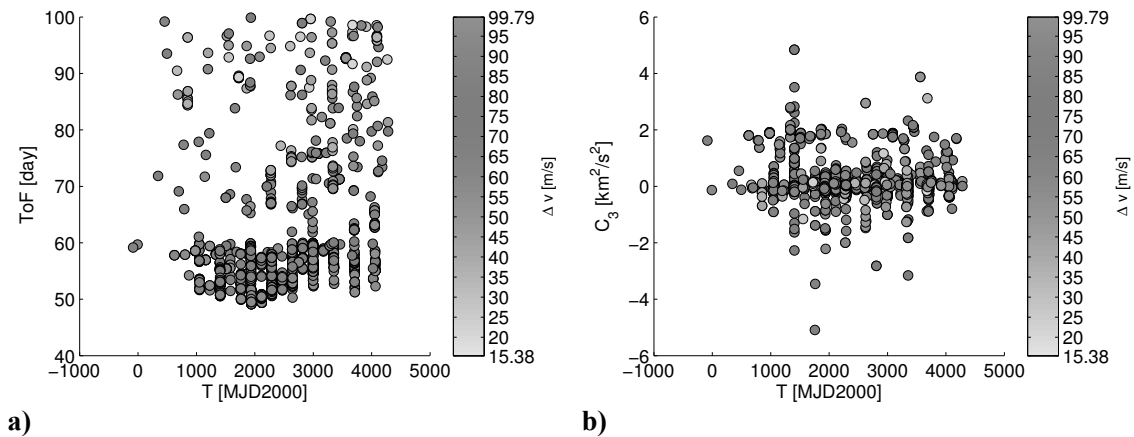
Figure 10. A) Time of flight and b) C_3 value to impact the Moon as a function of the time of departure from the SOHO LPO in MJD2000. Solutions are colour-coded according to the \Delta v cost in m/s.
