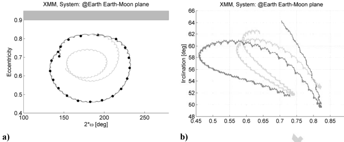
Figure 6. XMM graveyard disposal manoeuvre in 2016: Phase space evolution in the eccentricity- 2\omega -inclination phase space (Earth-Moon plane) a) 2\omega -eccentricity and b) eccentricity-inclination. Red: nominal predicted orbit, black lines: \Delta v manoeuvre. The light blue line represents the evolution of the orbital elements with respect to the Earth-Moon plane after the disposal manoeuvre is performed for the following 30 years.
