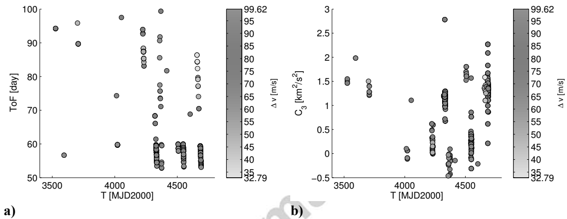
Figure 9. A) Time of flight and b) C_3 value to impact the Moon as a function of the time of departure from the Herschel LPO in MJD2000. Solutions are colour-coded according to the \Delta v cost in m/s.
