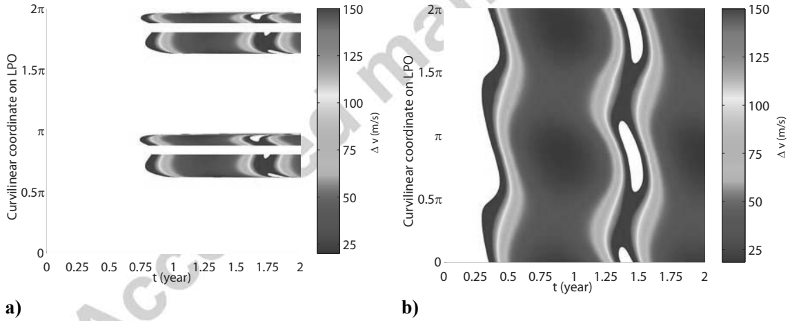
Figure 12. \Delta v cost for Herschel mission to close the surfaces of Hill as function of the time after departure from the LPO and position of departure on the LPO. Disposal towards a) the inner part of the solar system and b) the outer part of the solar system.
