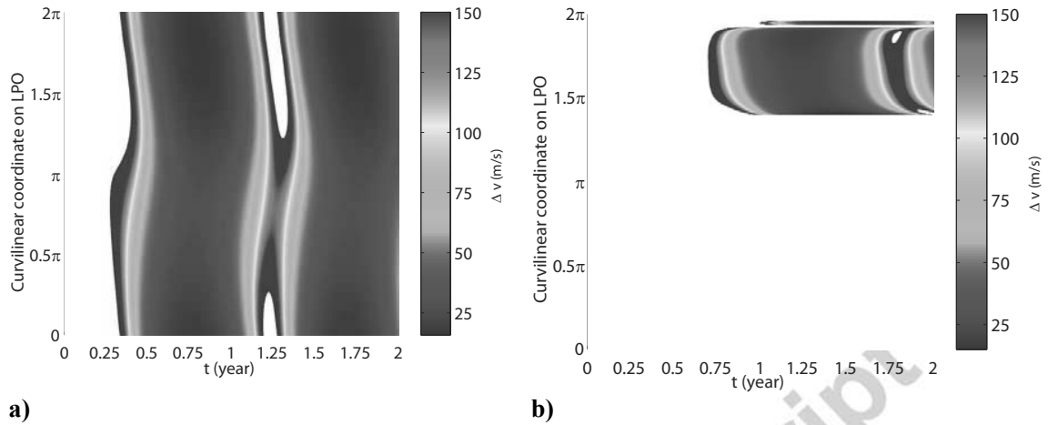
Figure 13. \Delta v cost for SOHO mission to close the surfaces of Hill as function of the time after departure from the LPO and position of departure on the LPO. Disposal towards a) the inner part of the solar system and b) the outer part of the solar system.
