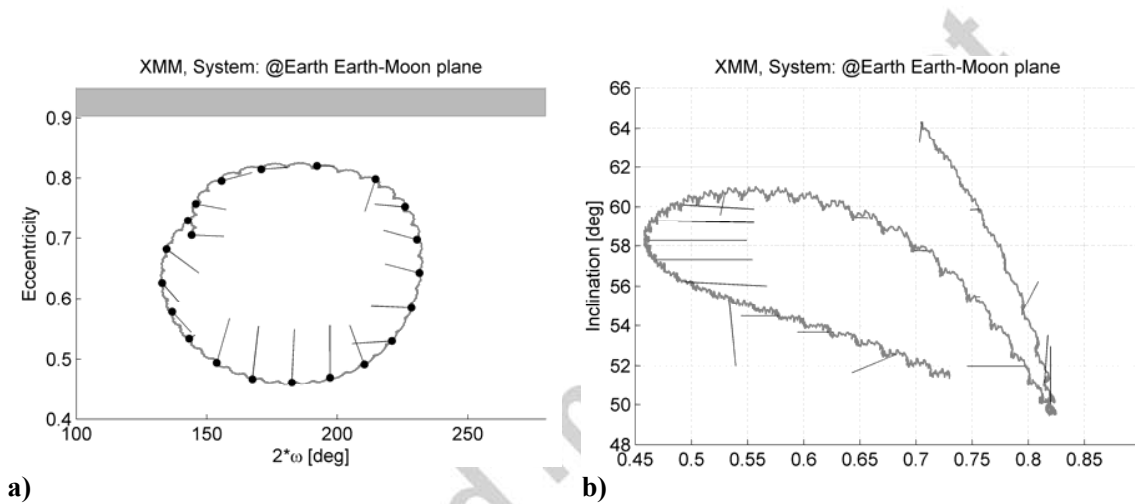
Figure 5. XMM graveyard disposal manoeuvres between 2013 and 2033: Phase space evolution in the eccentricity- 2\omega -inclination phase space (Earth-Moon plane) a) 2\omega -eccentricity and b) eccentricity-inclination. Red: nominal predicted orbit, black lines: \Delta v manoeuvres. The shaded area indicates eccentricities beyond the critical eccentricity for re-entry (at perigee altitude of 50 km).
