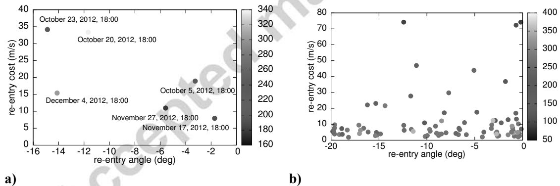
Figure 7. Re-entry feasible solutions. A) Herschel mission: the colour bar refers to the total time of flight (days) from the libration point orbit to the Earth. B) SOHO mission: the colour bar indicates the starting date on the LPO for the re-entry (years from J2000).
