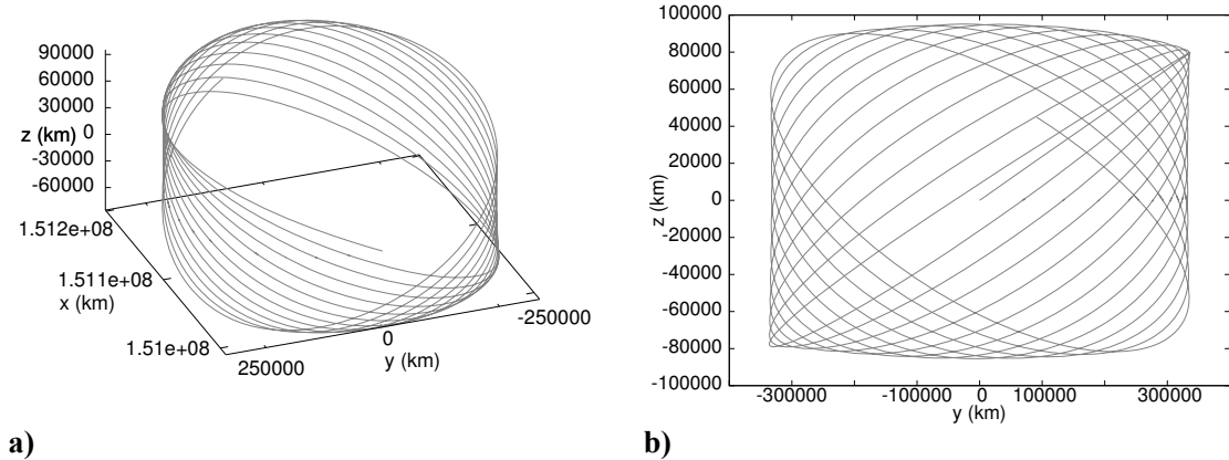
Figure 2. Lissajous orbit selected to simulate the evolution of Gaia. Synodic reference system centred at the Sun – Earth + Moon barycentre. A) 3D representation and b) y-z projection.
