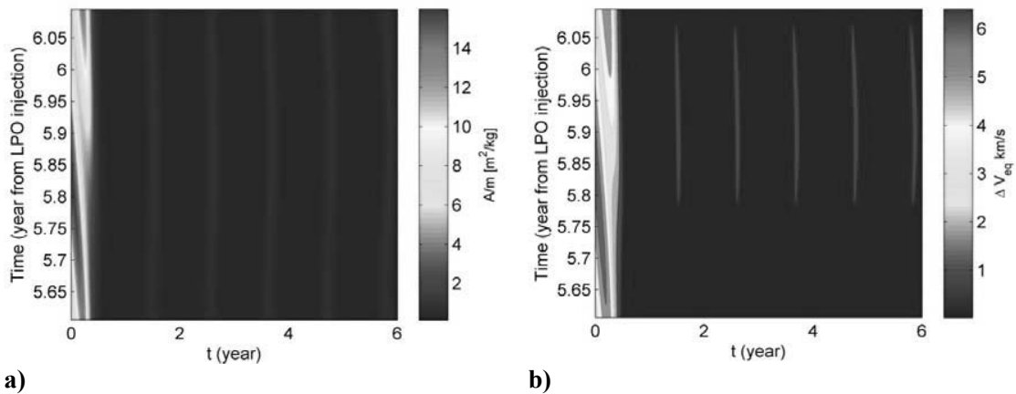
Figure 15. Gaia disposal through SRP. A) Required area-to-mass ratio for the closure of the Hill's curves and b) equivalent \Delta v .
