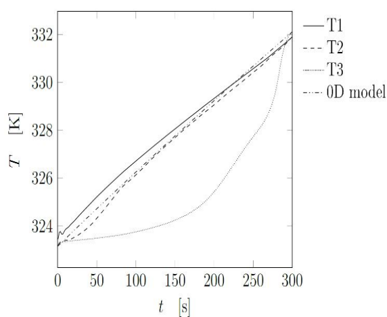
Figure 3 Temperature profiles of measuring devices for LR and 0D models for Case 1 in the first 300s of simulation.
