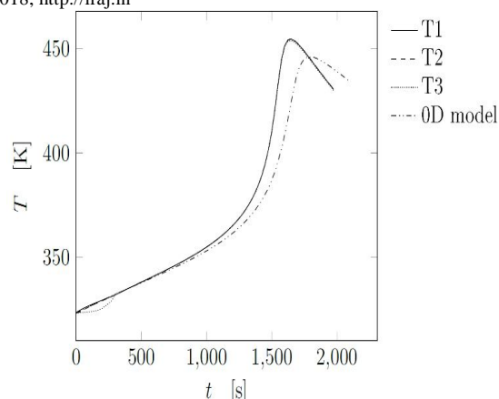
Figure 2 Temperature profiles of measuring devices for LR and 0D models for Case 1.
