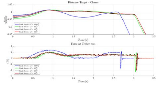
Figure 16 – Stabilization Phase: relative distance and tether tension for different tether slacks
