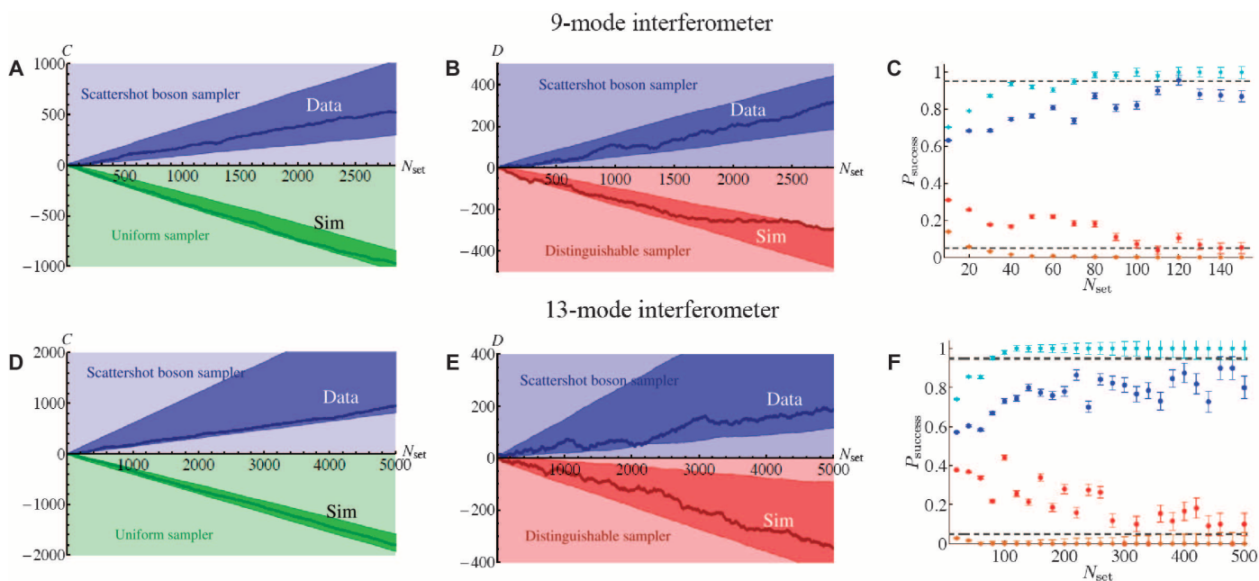
Fig. 4. Validation of multiple-input and scattershot boson sampling against various alternative distributions. (A and D) Application of the Aaronson and Arkhipov test against the uniform distribution (A: for the 9-mode chip; D: for the 13-mode chip). (B and E) Application of the likelihood ratio test against distinguishable sampler (B: for the 9-mode chip; E: for the 13-mode chip). (C and F) Success probability P_{\text{success}} of the validation protocol against different alternative distributions as a function of the data set size N_{\text{set}} (C: for the 9-mode chip; F: for the 13-mode chip). Horizontal dashed line: 0.95 and 0.05 thresholds for the success probability P_{\text{success}} . (A, B, D, and E) Blue points, scattershot boson sampling experimental data; green points, numerical simulation of a uniform sampler; red points, numerical simulation of distinguishable sampler data; dark
