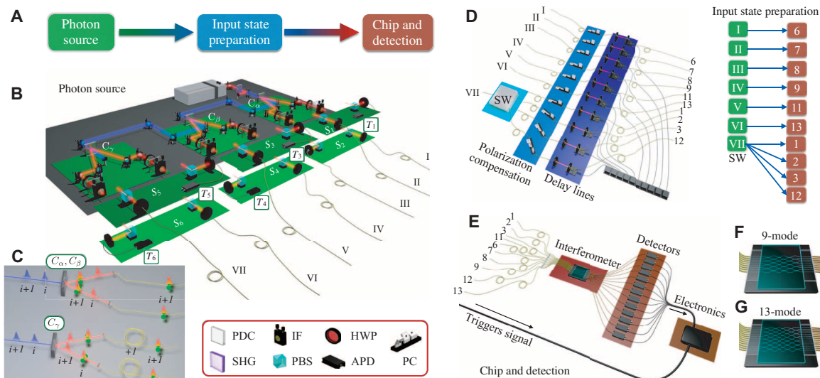
Fig. 2. Experimental layout for the implementation of boson sampling with multiple inputs. (A) Overall conceptual scheme of the experiment. (B) In each of the three BBO crystals ( C_\alpha , C_\beta , and C_\gamma ), photon pairs are generated via type II PDC process. The two possible polarization combinations for the two generated photons, HV and VH, constitute two equal PDC sources enfolded in the same crystal, each one exciting a different trigger (photon V) and a different input mode (photon H). The only exception is given by source S_2 , whose outputs (I and III in the figure) are both injected in the chip. Sources are also time-multiplexed, because pulses generating photons in crystal C_\gamma are produced before the ones generating photons in C_\alpha and C_\beta . (C) Schematic visualization of the six time- and space-multiplexed photon sources; i is an index of the pump pulse number. (D) For the nine-mode device, the input state is varied manually by changing
