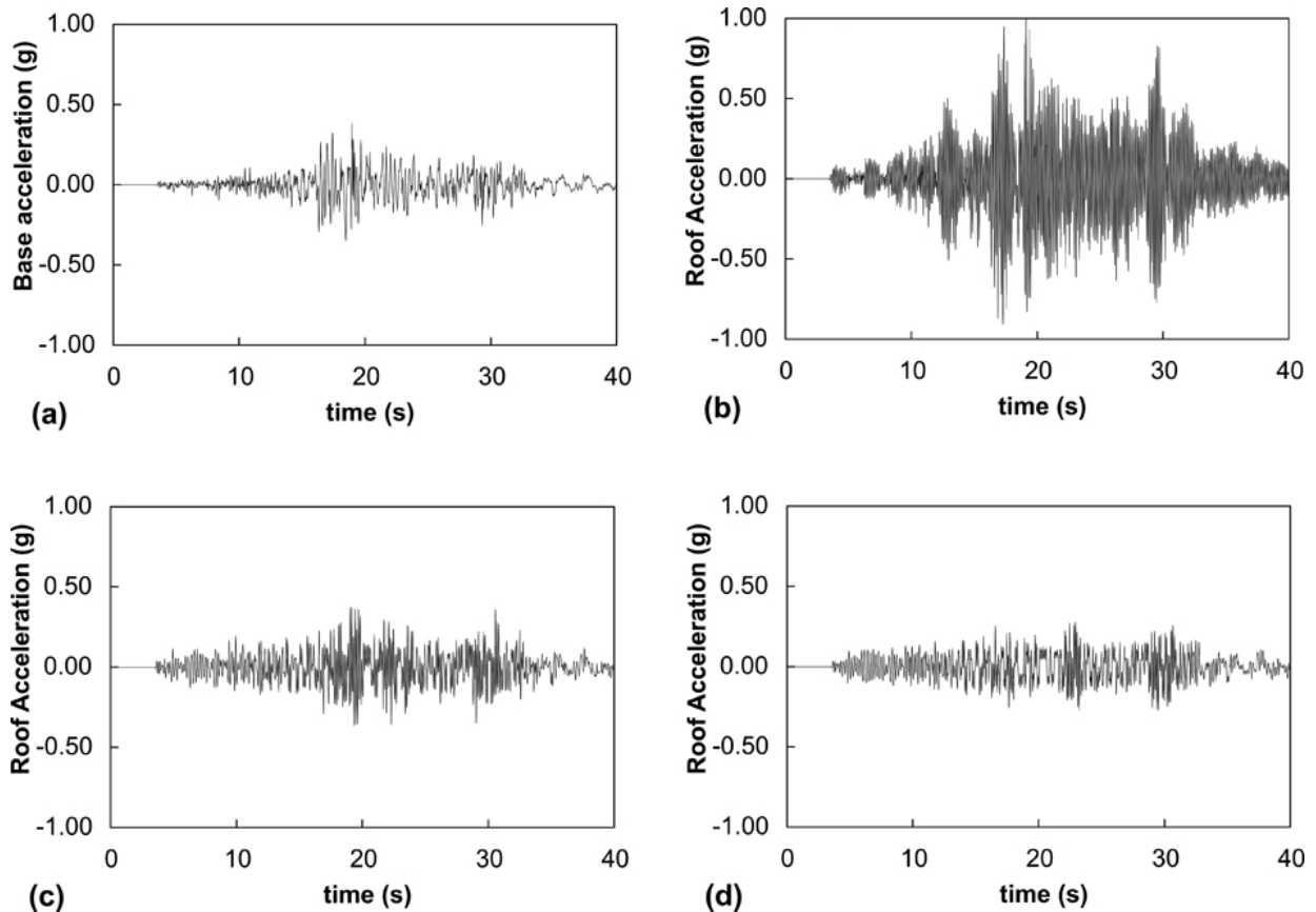
Fig. (5). (a) Ground motion, roof acceleration of: (b) non-isolated model; (c) marble-HDPE model; (d) marble-marble interface.
