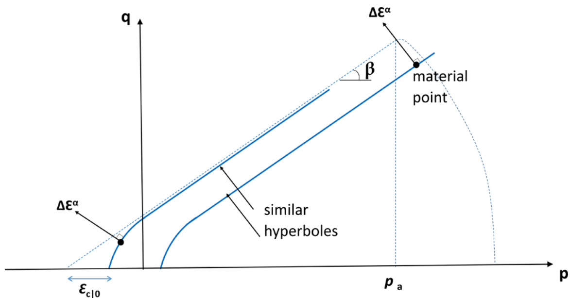
Fig. (4). Smoothed Drucker-Prager failure criterion adopted in the simulation, p - q plane.
