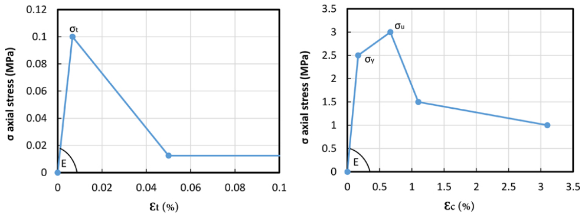
Fig. (2). ABAQUS material non-linear behavior in uniaxial tension and compression.
