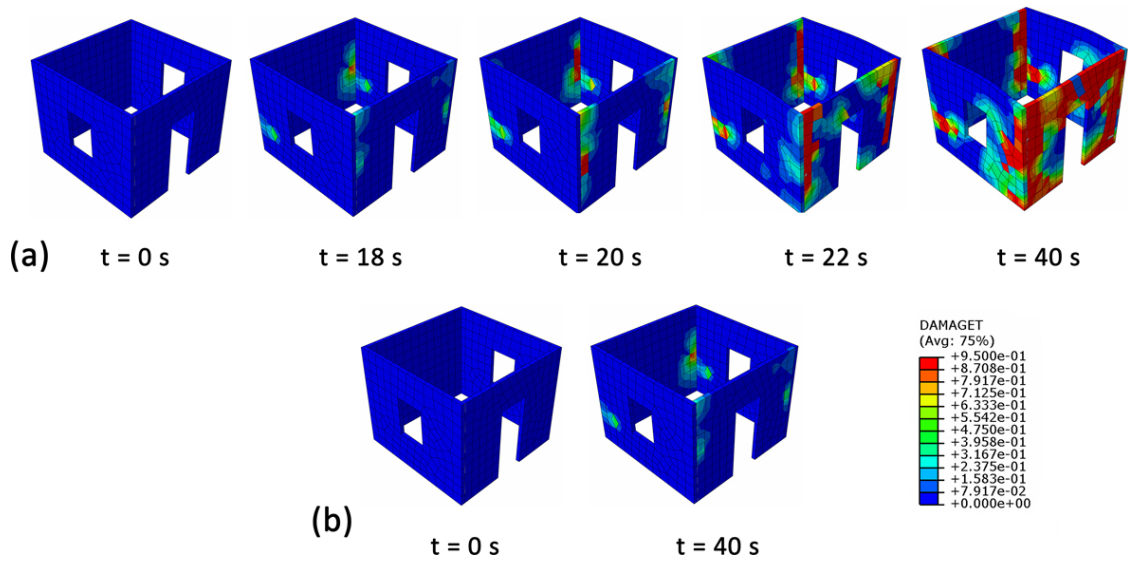
Fig. (6). Tensile damage propagation during ground motion, (a) Model without isolation, (b) all models with base-friction isolation.
