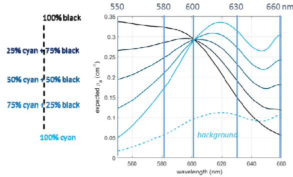
Fig.1 Spectra of the multichromophore “balloon” inclusions
