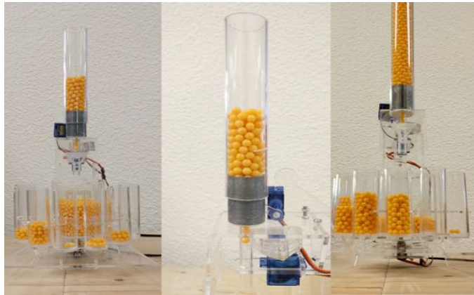
Fig. 7. The working prototype of the Budgy
