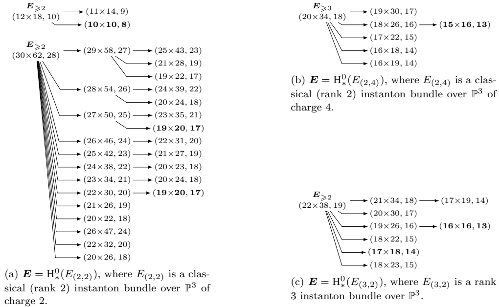
FIGURE 4. Examples of possible constant rank matrices that can be obtained from instanton bundles. The notation is the same as in Figure 3.
