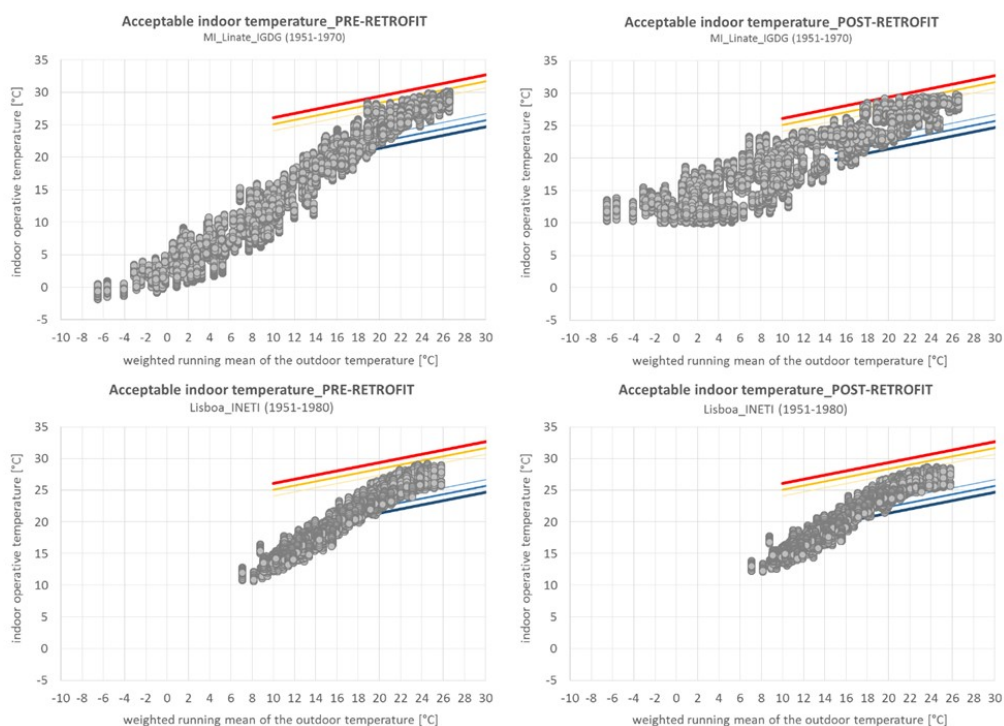
Fig. 3. Comfort analysis under free-floating condition for the baseline and retrofit scenario
