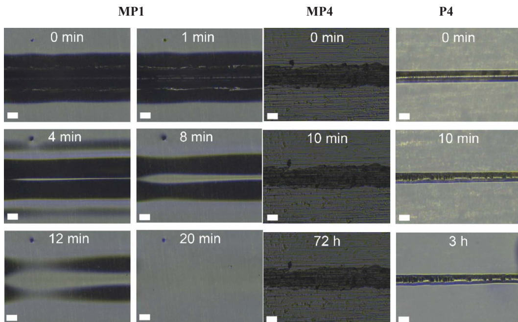
Fig. 3. Optical micrographs showing scratch healing in MP1, MP4 and P4 at 100 °C. Scale bars are 100 \mu m.
