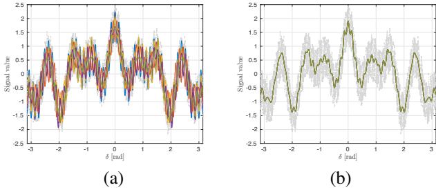
Fig. 2. Data points (grey crosses), and the functions (solid lines) corresponding to the local solutions returned by Algorithm 1 (a) at the initialization and (b) after 150 iterations.
