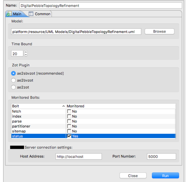
Figure 5: Run configuration view.
