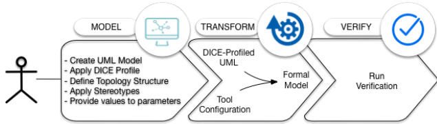
Figure 3: The main steps of D-VerT workflow.
