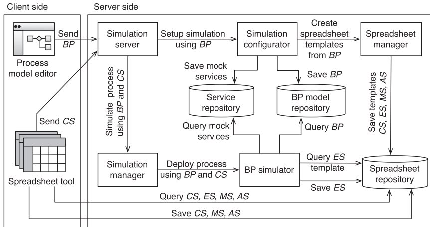
Fig. 8. Architecture of the proposed solution.
