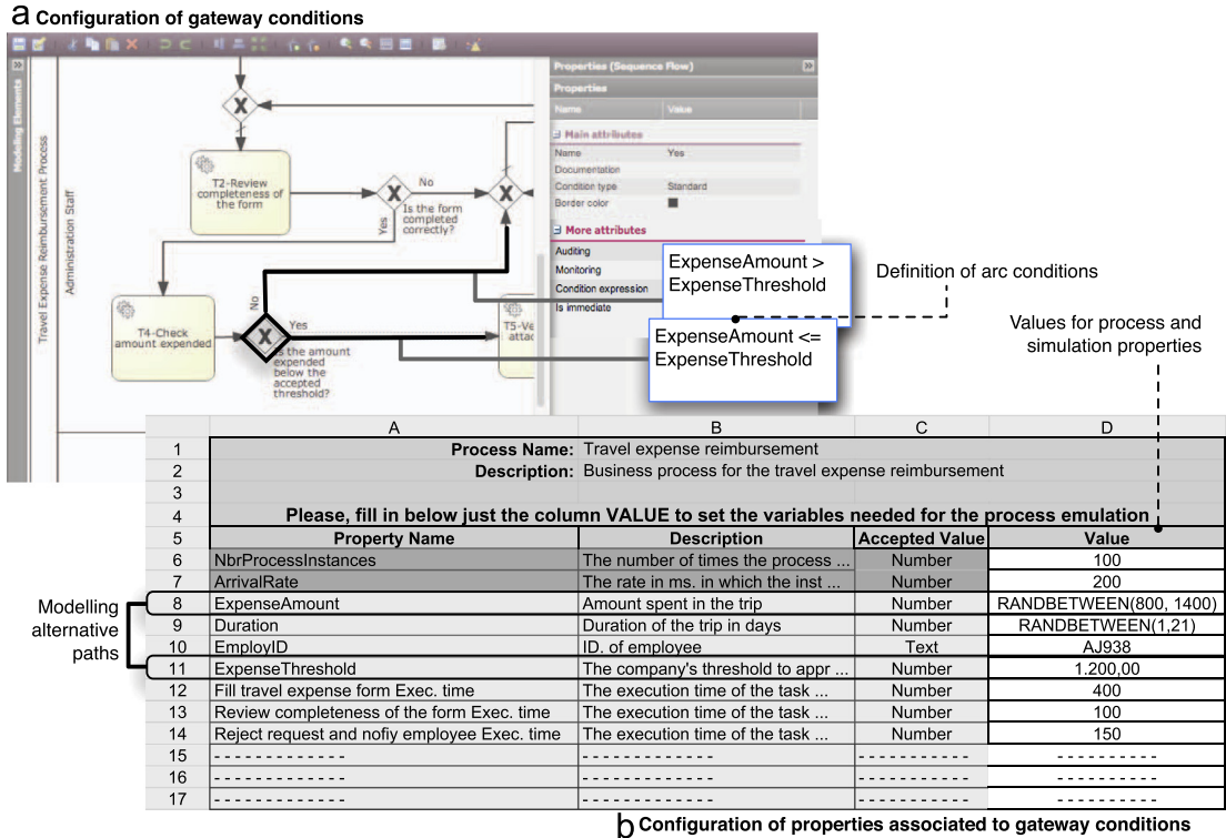
Fig. 5. Modelling and configuring gateway nodes.
