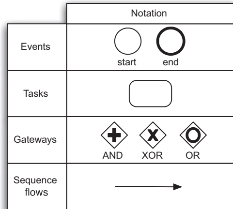
Fig. 2. BPMN elements related to control-flow specification.
