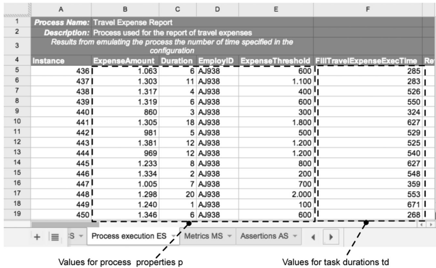
Fig. 6. Process execution spreadsheet ES containing logged process progression information.
