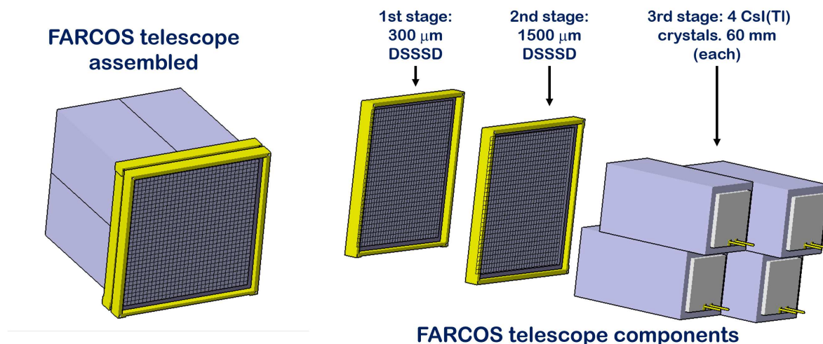
Figure 1. FARCOS telescope composition. Left image shows one of the FARCOS telescope assembled, while in the image on the right are show the components of each telescope: two DSSSD 300 and 1500 \mu\text{m} thickness respectively, and 4 CsI(Tl) crystals (60 mm each) at back, covering the same active area than the silicon detectors ( 64 \times 64 \text{ mm}^2 ).
