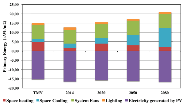
Fig. 6. Primary energy breakdown of the post-retrofit building including electricity generated by the PV system.
