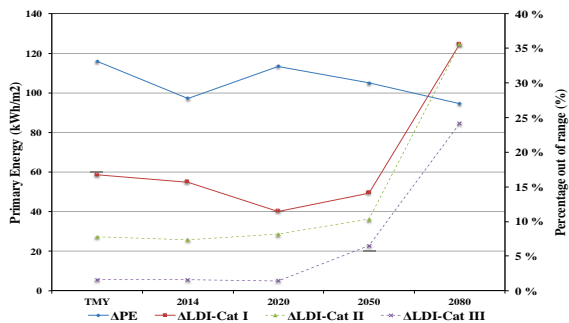
Fig. 5. Difference of primary energy usages (ΔPE) and absolute difference of long-term discomfort index (ΔLDI) of pre- and post-retrofit models
