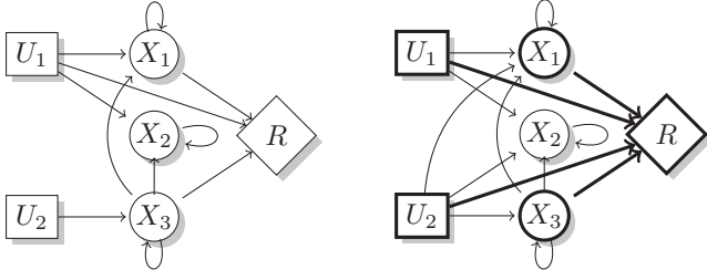
(a) Graph representation of the adjacency matrix \Sigma . (b) Graph representation of the transitive closure \Sigma^+ .
