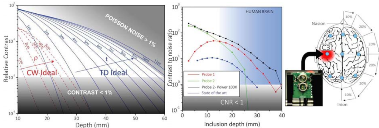
Fig. 1. (left) Simulation of the contrast produced in a realistic case using ideal CW and TD systems. (centre) Experimental results on contrast-to-noise ratio obtained using TD probes. (right) Probe positioning example for functional brain imaging.
