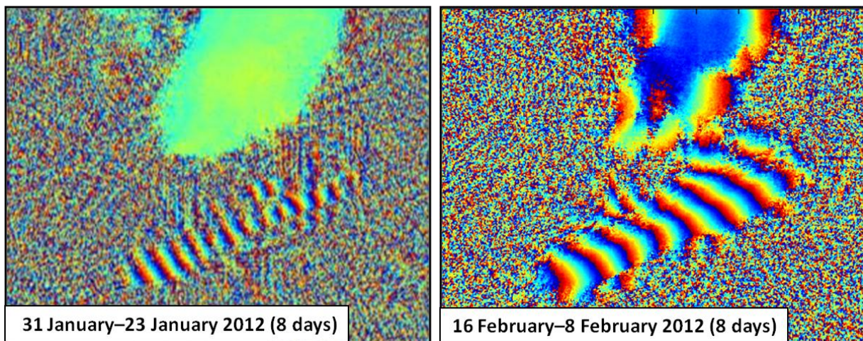
Figure 3. Example of interferograms obtained for the Costa Concordia interferometric analysis. It is possible to notice how interferometric fringes change over time when considering a similar temporal interval.
