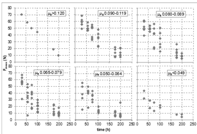
Figure 2: Fruit firmness in function of time at 20°C for different levels of \mu_a measured at harvest.
