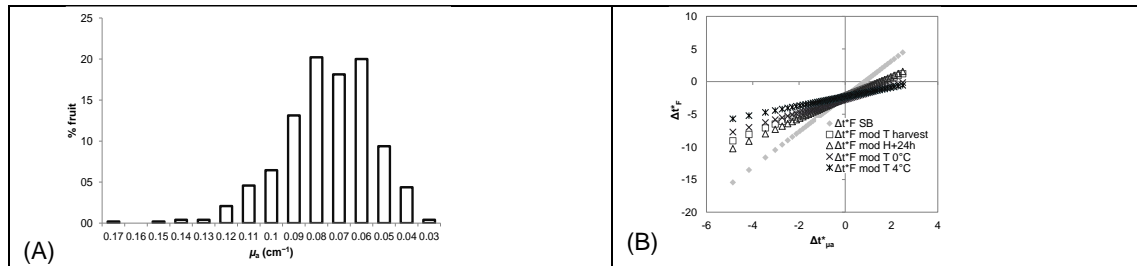
Figure 1: (A) Percentage distribution of absorption coefficient at 670 nm measured at harvest (480 fruits). (B) Plot of BSF for firmness in function of BSF for \mu_a for ‘Morsiani 90’ in comparison to ‘Spring Bright’ cultivar (SB, Rizzolo et al., 2009).
