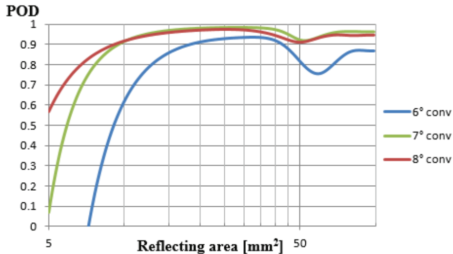
FIGURE 8. MAPOD curves for 6°, 7° and 8° convergent transducers.
