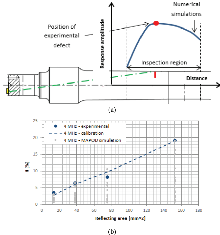
FIGURE 2. Traditional calibration of the rotating probe and its problems.
