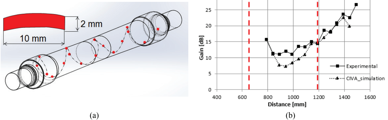
FIGURE 3. Ultrasonic inspection of the novel sample block ( 6^\circ convergent transducer).
