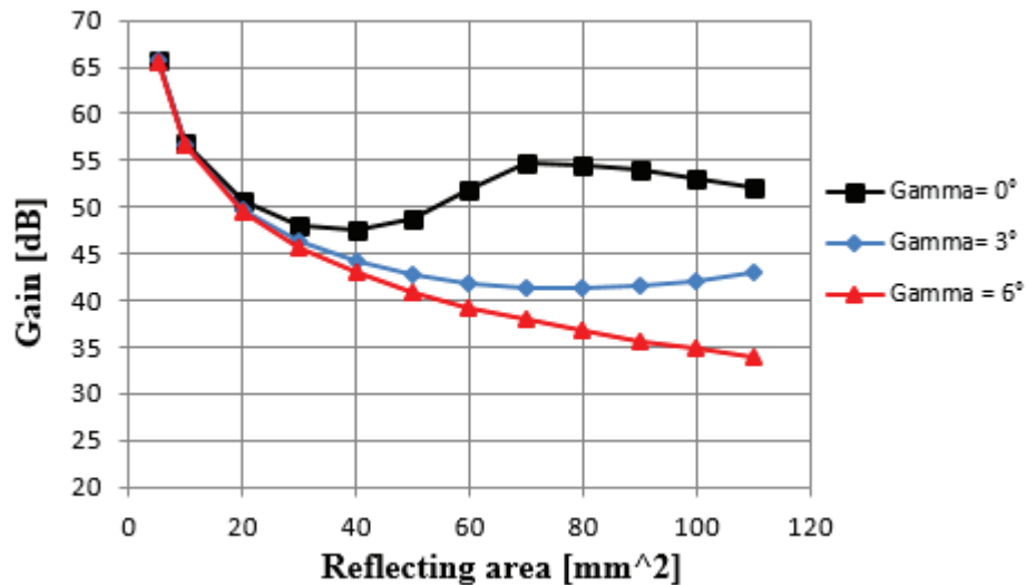
FIGURE 7. Trend of ultrasonic responses with the reflecting area of defects.
