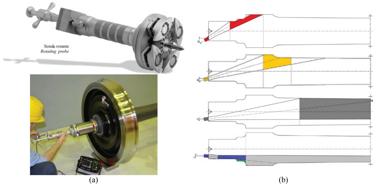
FIGURE 1. Rotating probe for ultrasonic inspection of solid axles.
