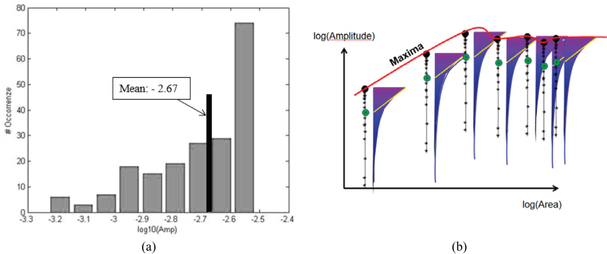
FIGURE 6. Statistical analysis of rotating probe UT responses.
