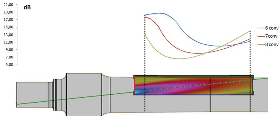
FIGURE 4. Analysis of the sound pressure field for different refraction angles.
