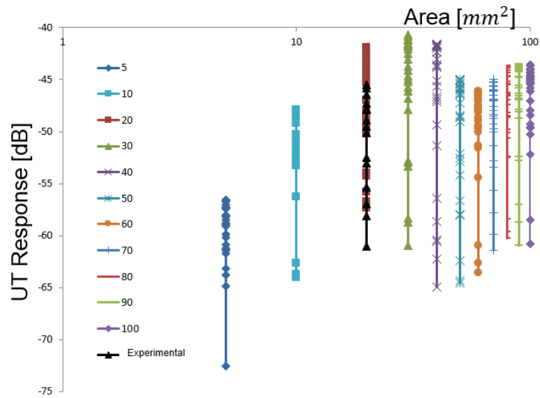
FIGURE 5. MAPOD analysis for the 6° convergent transducer.
