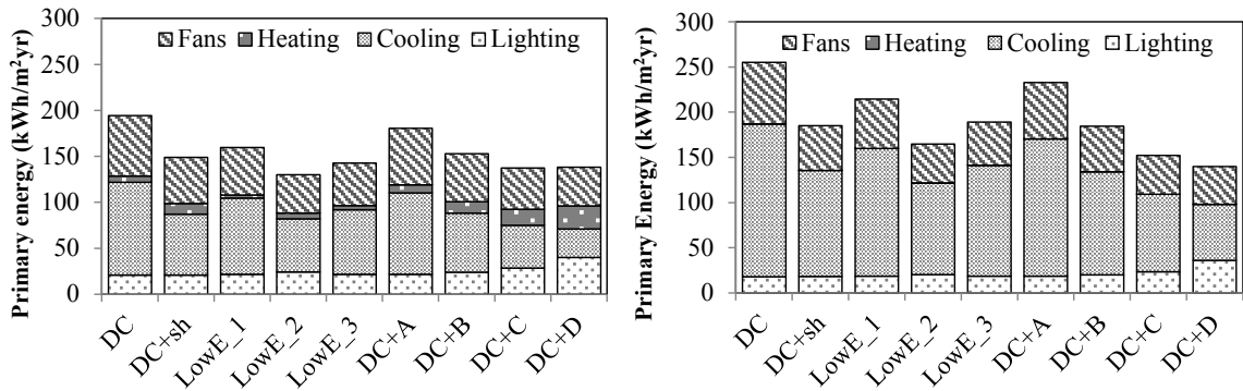
Fig. 4. Primary energy use comparison for Fans, Heating, Cooling and Lighting for the proposed retrofit solutions in Milan (a) and Palermo (b). -ribbion window- Window to wall ratio 50%.
