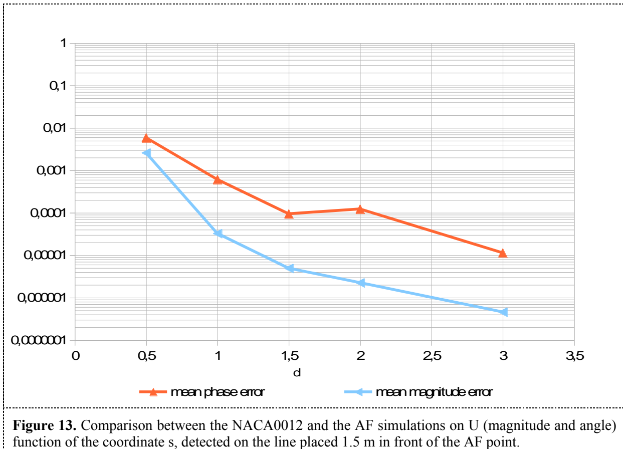
Figure 13. Comparison between the NACA0012 and the AF simulations on U (magnitude and angle) function of the coordinate s , detected on the line placed 1.5 m in front of the AF point.
