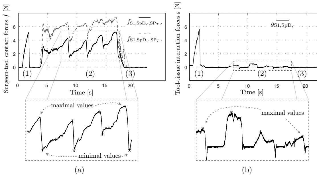
Figure 4: Example of displacement test with spatula (SpD) performed by S1. (a)-upper figure: surgeon tool contact forces measured by the contact sensors: continuous and dotted line represent the thumb f_{S1,SpD,.,SP_T,} and the index sensor f_{S1,SpD,.,SP_I,} measurements. (a)-lower figure: magnification of (a)-upper figure: interaction phase, stars and crosses represent the maxima and the minima selected in the trial, respectively. (b) tool-tissue interaction forces measured by the load cell: the continuous line represents the measurements of the tool-tissue interaction forces g along the \hat{x}_T axis of the spatula tool. (b)-lower figure: magnification of (b)-upper figure: interaction phase, stars represent the maxima selected in the trial. Both figures: (1) synchronization phase, (2) interaction phase, (3) resting phase. In (1), force spikes used for the offline synchronization of the signals are visible.
