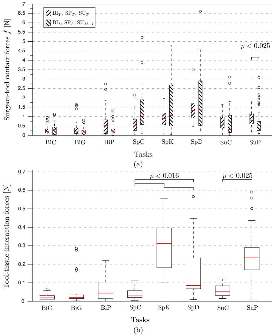
Figure 5: Surgeon-tool contact forces and tool-tissue interaction forces: (a) measurements from the contact force sensors pressed by the thumb, i.e., BI_T , SP_T , and SU_T , and by the index and middle fingers, i.e., BI_I , SP_I , and SU_{M-I} , expressed in N, collected by tasks; (b) measurements from the load cell, expressed in N, collected by tasks. Both figures: for each task, the medians, the 25 th and the 75 th percentiles of the samples, the whiskers for the minimal and maximal values are shown. Outliers are depicted with circles. Significant differences between medians are marked with horizontal brackets.
