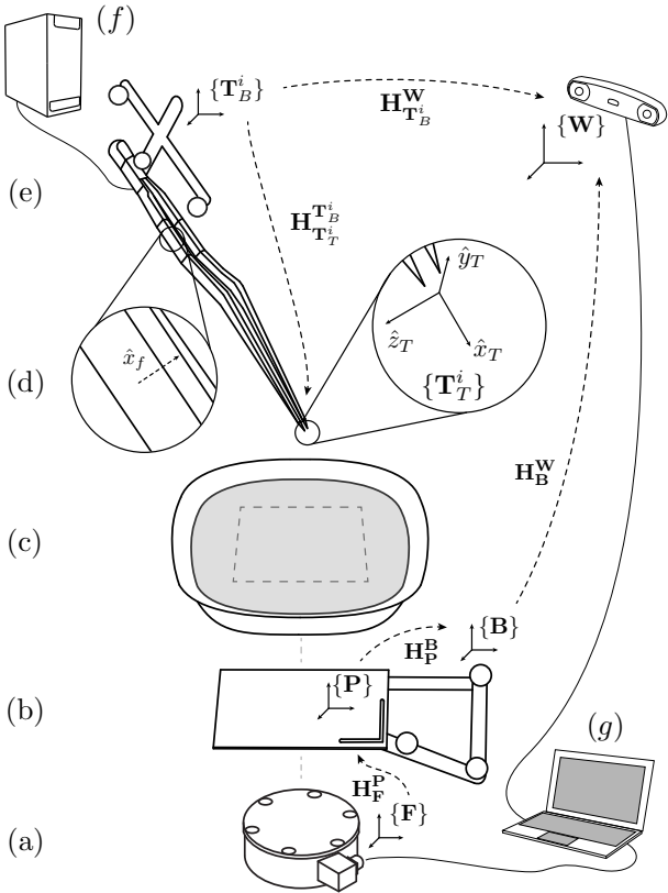
Figure 1: The acquisition setup was composed by a (c) soft tissue mimicking phantom placed over a (b) Acrylonitrile Butadiene Styrene (ABS) 3-D printed plate, fixed over a (a) six DoFs force/torque load cell. The ABS 3-D printed plate and each tool (e) were localized with passive retro reflective optical markers. Tools were instrumented with (d) contact force sensors, whereas the underlying load cell acquired the force exerted to the brain phantom. The (f) PC 1 was used for the contact force sensors measurements acquisition, while (g) PC 2 for the optical localization system and load cell measurements acquisition. Load cell reference frame \{\mathbf{F}\} , ABS base reference frame \{\mathbf{P}\} , ABS passive optical markers reference frame \{\mathbf{B}\} , world reference frame \{\mathbf{W}\} (which is also the optical localization system reference frame), i^{th} tool passive optical markers reference frame \{\mathbf{T}_B^i\} , i \in \mathbb{T} , contact forces sensor reference axis \hat{x}_f , i^{th} tool tip reference frame \{\mathbf{T}_T^i\} , and all the homogeneous transformation \mathbf{H} are shown.
