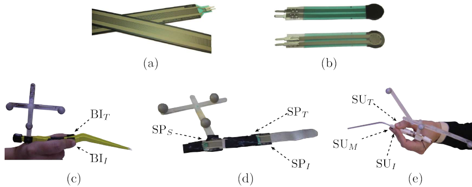
Figure 2: Upper row: Force Sensitive Resistors fixed on the surgical tools, (a) FSR TM 408 series, (b) FSR TM 400 series. Lower row: instrumented surgical tools, (c) bipolar forceps, (d) spatula, (e) suction tool. The contact force sensors are indicated by dotted arrows. BI T and BI I are the contact force sensors on the bipolar forceps at the contact points of the thumb and of the index, respectively. SP T , SP I , and SP S are the contact force sensors on the spatula at the contact points of the thumb, of the index, and of the side sensor, in fact not active, respectively. SU T , SU I , and SU M are the contact force sensors on the suction tool at the contact points of the thumb, of the index, and of the middle finger, respectively.
