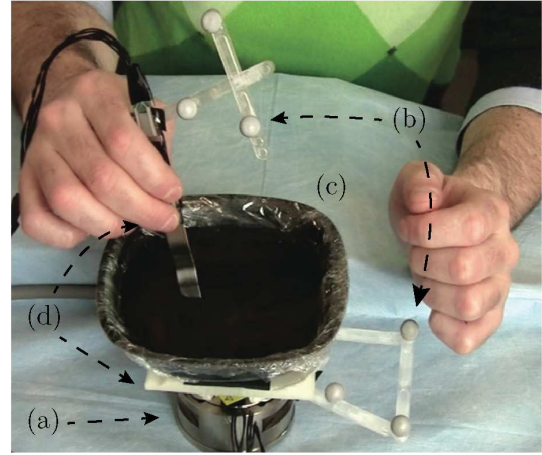
Figure 3: Setup for interaction forces acquisition. The surgeon is performing the cut test with spatula (SpK). The (a) multi-axis load cell, the (b) passive optical markers on the tool and on the ABS plate base, and (c) the brain phantom are visible, whereas the (d) ABS plate and the contact force sensors are partially occluded.
