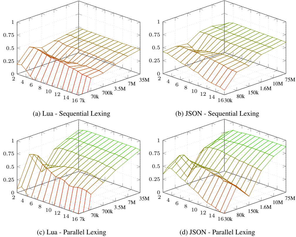
Figure 14: Parallel code portion in both the JSON and Lua lexing/parsing process obtained as the complement to the sequential code portion obtained via Karp-Flatt metric, plotted as a function of the number of workers, and the size of the input expressed in bytes.
