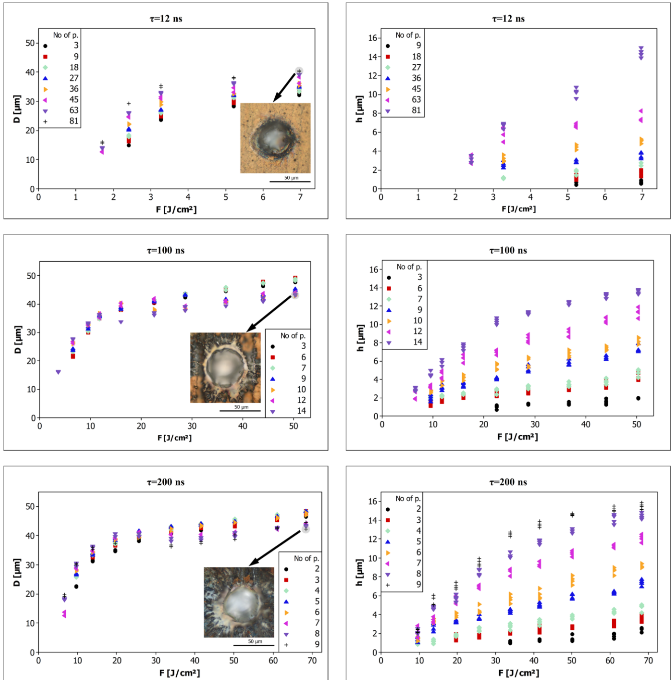
Figure 7. Hole diameters and depths as functions of the fluence and number of pulses for different pulse durations.
