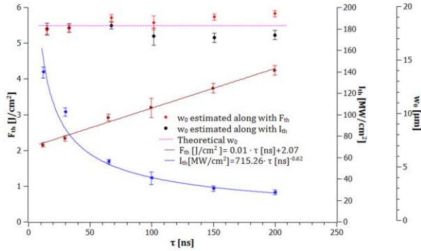
Figure 4. The results of the single-pulse ablation study: changes in the fluence and irradiance thresholds as functions of pulse duration; the theoretical value of the laser beam radius ( w_0 ); the estimated values for the laser beam based on the non-linear regression method and values of threshold fluence ( F_{th} ) and irradiance ( I_{th} ) for different pulse durations. The error bars represent the 95% confidence interval for the mean.
