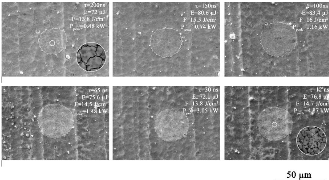
Figure 1. The shape characteristics of the different pulse durations.
