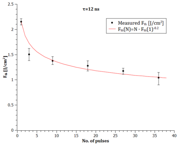
Figure 8. The fluence threshold as a function of the number of pulses for pulse duration of 12 ns. The error bars represent the 95% confidence interval for the mean.
