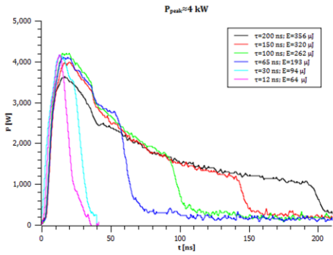
Figure 1. The shape characteristics of the different pulse durations.
