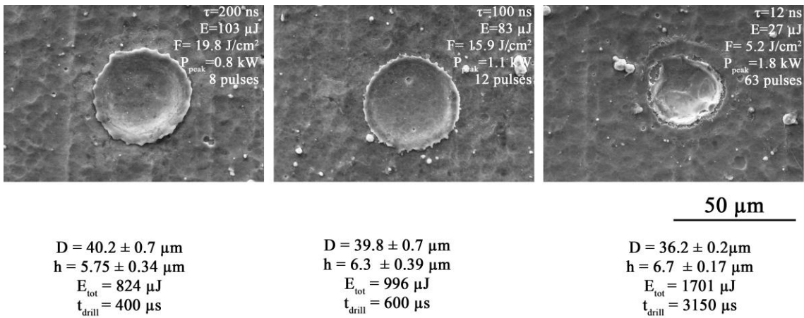
Figure 6. A comparison of holes with similar geometric properties obtained with different pulse durations, energy levels and number of pulses.
