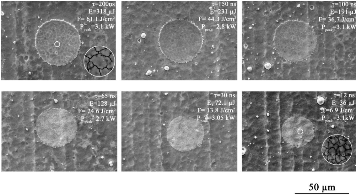
Figure 3. The evolution of ablated zones with similar peak power ( P_{peak} ) levels and different pulse durations. The small circles in the ablated regions with pulse durations of 200 ns and 12 ns are reported in higher magnification insets to show the crack dimensions. The diameter of the magnified region is 7.7 \mu m.
