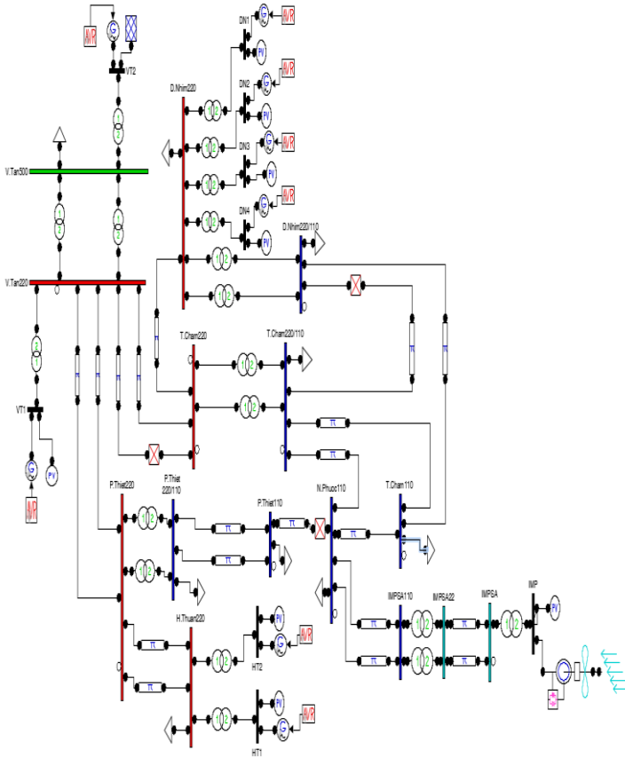
Figure 4. Ninh Thuan – Binh Thuan24 test system
