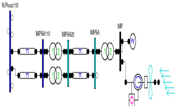
Figure 4. Ninh Thuan – Binh Thuan24 test system
