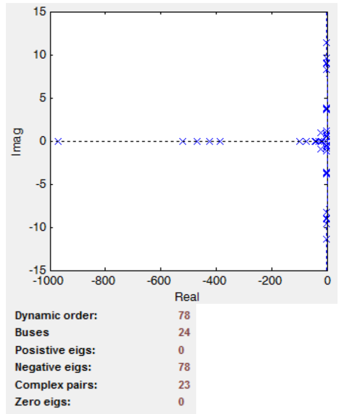
Figure 6. S-Domain analysis graphical representation of Ninh Thuan – Binh Thuan24 test system
