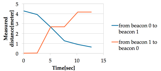
Figure 8. Signal dynamic evaluation (Coeff = 0.65)
