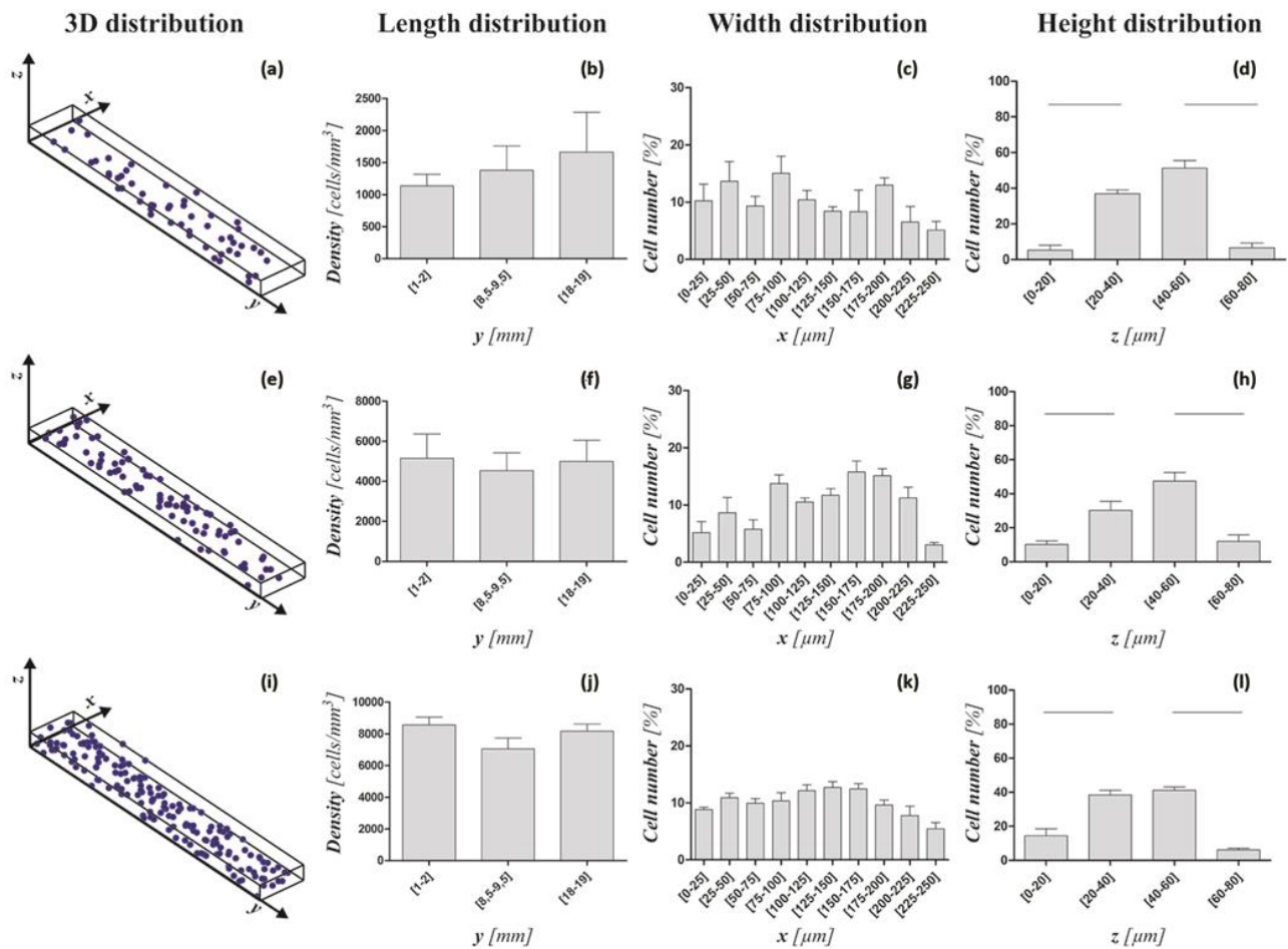
Figure 4. Cells spatial distribution. Positions of cell nuclei geometrical centers at densities of 1, 5 and 10 x 10 6 cell ml -1 were plotted from data obtained by analyzing confocal images of the DAPI stained cell-laden micropatterns at day 0. Cells were uniformly distributed along the channels length ((b), (f) and (j)) and width ((c), (g) and (k)). While a higher cell density was detected in the two central bands (l=20 \mu m) of the channels height ((d), (h) and (l)), the overall cell distribution resulted 3D uniform within the micropatterns ((a), (e) and (i)). (Error bars: \pm SD; n=3. All the reported comparisons are statistically significant for p<0.05).
