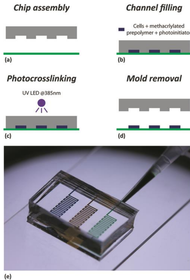
Figure 1. Photo-Mold Patterning (PMP) protocol. (a) The PDMS microfluidic mold is placed against a 3-(trimethoxysilyl) propyl methacrylate (TMSPPMA) treated slide. (b) Hydrogel prepolymer is injected into the channels, and (c) the photopolymerization is achieved using a commercial LED emitting at 385nm. (d) Upon PDMS removal, the 3D patterns are revealed on the glass substrate. (e) An example of PMP is reported, where three mold channels were independently filled with different colors.
