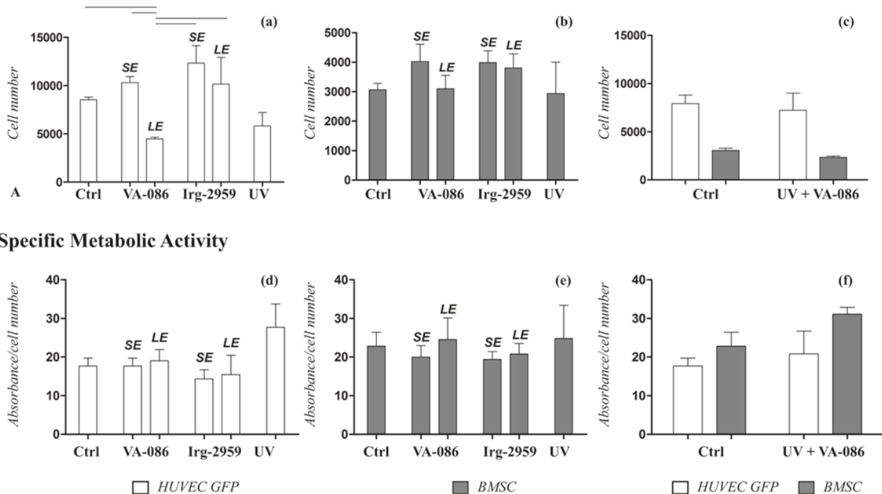
Figure 3. PI and UV cytotoxicity analyses. HUVEC GFP and BMSC 2D cultures were subjected to different photocrosslinking treatments to assess the PMP cytocompatibility. Single and combined effects of Short Exposure (SE, 4hr) and Long Exposure (LE, 24hr) inactive PI molecules (VA-086 and Irg-2959) and UV ( \lambda=385\text{nm} for 3min) were tested 24 hours after the treatments. ((a), (b), (d) and (e)). For both cell types, the presence of both the PI molecules and the exposure to UV didn't cause any statistically significant reduction in cell number and specific metabolic activity compared to control. A reduction in HUVEC GFP number was detected for VA-086 LE though maintaining a high specific metabolic activity. ((c) and (f)) The combination of VA-086 and UV resulted favorable in terms of cell viability demonstrating the biocompatibility of PMP protocol. (Error bars: \pm\text{SD} ; n=5 . All the reported comparisons are statistically significant for p<0.05 ).
