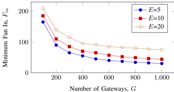
Fig. 7. Minimum Gateway fan-in to guarantee that the heuristic algorithms provide a feasible solution for more than 50% of the instances, assuming M=5000 . The precision of the confidence intervals (omitted in the plot) is below 10%.
