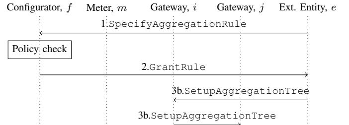
Fig. 4. Configuration phase of the SSS-based aggregation protocol with distributed routing
