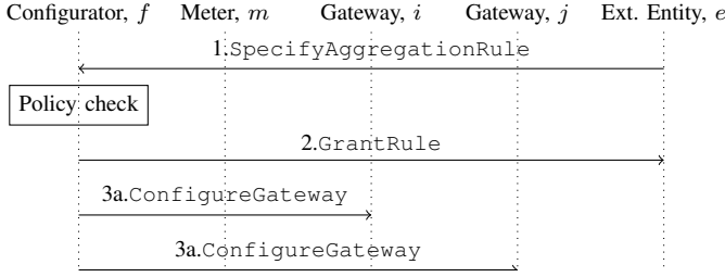
Fig. 3. Configuration phase of the SSS-based aggregation protocol with centralized routing
