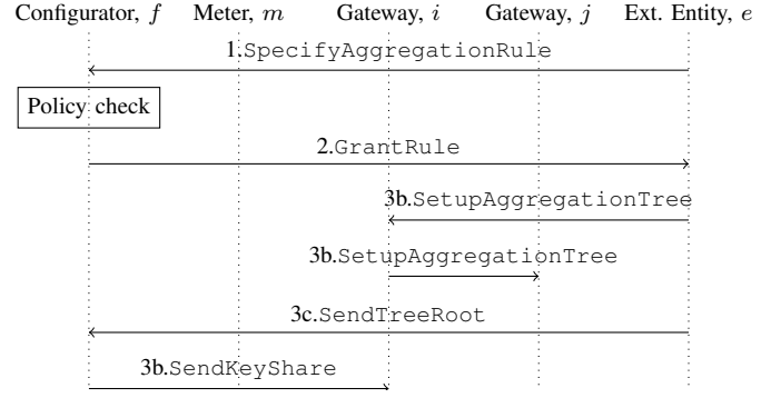
Fig. 6. Configuration phase of the CS-based aggregation protocol with distributed routing
