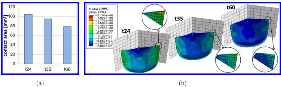
Fig. 3. Computational outcomes as a function of the leaflet thickness: (a) Coaptation area; (b) Von Mises stress [MPa].
