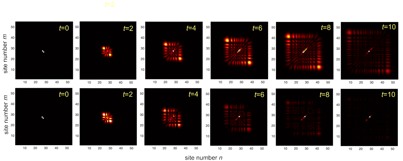
FIG. 6. Temporal evolution of the two-particle probability distributions |\psi_{n,m}(t)|^2 in a lattice with the same parameter values as in Fig.5 ( J = 1, U = 10, V = 0.15, L = 55, \theta = 0 ) and for h = 0 (Hermitian limit, upper row) and h = 1 (lower row). The system is initially prepared in a symmetrized state with one particle at site n_1 = 26 and the other one at site n_2 = 27 .
