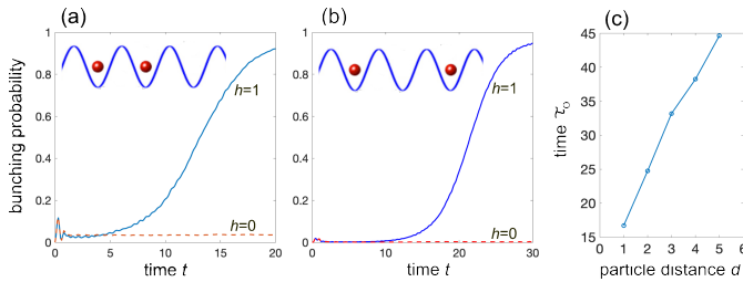
FIG. 7. (a) Temporal evolution of the bunching probability for the same parameter values as in Fig.6 for h = 0 (Hermitian limit, dotted curve) and h = 1 (solid curve). (b) Same as (a), but for an initial separation of the two particles d = 2 . (c) Behavior of the bunching time \tau_0 versus initial particle distance d for h = 1 . \tau_0 is defined such that P_{bun}(\tau_0) = 0.8 .
