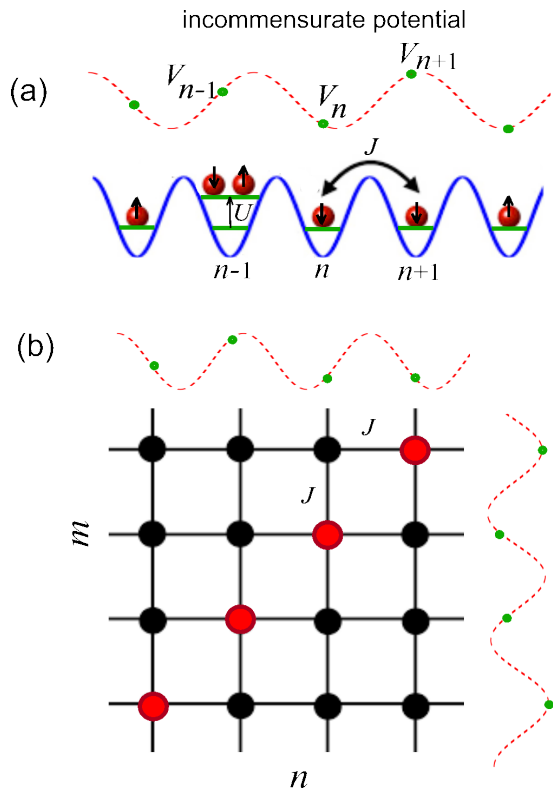
FIG. 1. (a) Non-Hermitian Hubbard model, describing correlated many-particle states in a one-dimensional lattice with a superimposed incommensurate on-site potential (quasi crystal). The reciprocal single-particle hopping rate between adjacent sites is J , U is the on-site interaction energy, and V_n = V \cos(2\pi\alpha n + \varphi) is the incommensurate potential with complex phase \varphi = \theta + ih . (b) The Hubbard model for two fermions with opposite spins can be mapped onto the dynamics of a single particle on a square lattice with a line defect on the main diagonal n = m (red circles), corresponding to the interaction energy U , and with a hopping rate J . States bound on the main diagonal n = m in (b) correspond to stucked two-particle states (doublons) in (a). In the strong interaction regime, doublons undergo correlated hopping via a second-order tunneling process with an effective hopping rate J_e \simeq 2J^2/U .
