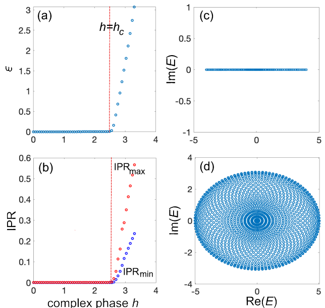
FIG. 2. Two-particle energy spectrum and IPR of eigenstates in the non-interacting limit U = 0 . Other parameter values are J = 1 , V = 0.15 , \theta = 0 , \alpha = 34/55 and L = 55 . (a) Behavior of the largest value \epsilon (in modulus) of the imaginary part of any eigenenergy versus the complex phase h of the incommensurate potential. The vertical dashed line corresponds to the spectral phase transition point h = h_c = \log(2J/V) \simeq 2.59 . (b) Behavior of the largest and smallest values of the IPR versus h . (c,d) Energy spectra in complex energy plane for h = 1 [panel (c)] and h = 3.3 [panel (d)]. In (d) the spectrum comprises multiple layers of closed loops in complex plane, characterized by a non-vanishing winding number w for any base energy E_B internal to such loops. For example, for the base energies E_B = 0, 1.5 and 2.5 one has w = -55, -45 and -37 , respectively.
