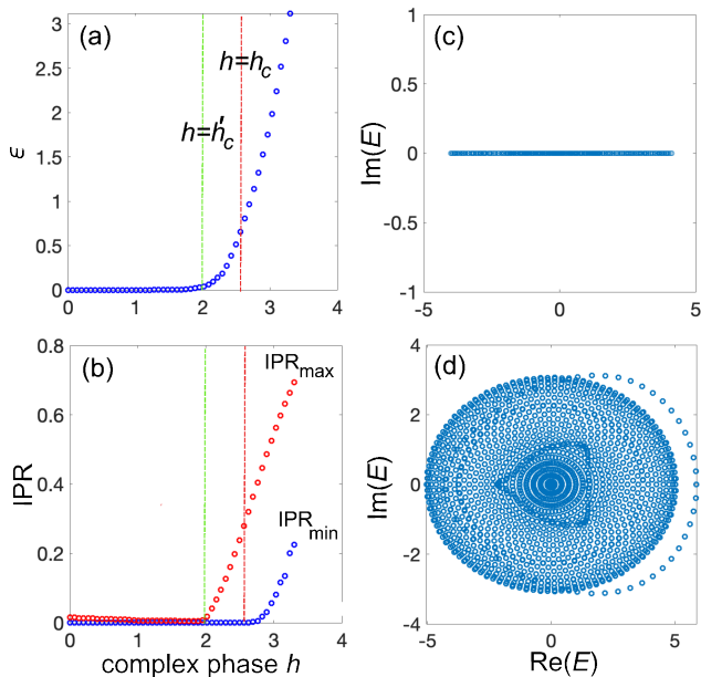
FIG. 3. Same as Fig.2, but for U = 1 . Note that the real-to-complex spectral phase transition is observed at a lower value h'_c of the complex phase than h_c . The value h'_c corresponds to the appearance of localized eigenstates, indicated by a finite value of \text{IPR}_{\max} . For h < h'_c all eigenstates are extended, for h'_c < h < h_2 with h_2 \simeq h_c localized and extended states coexist, whereas for h > h_2 all eigenstates are localized.
