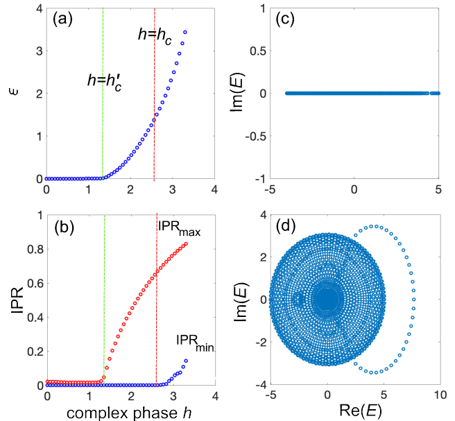
FIG. 4. Same as Fig.3, but for U = 3 .
