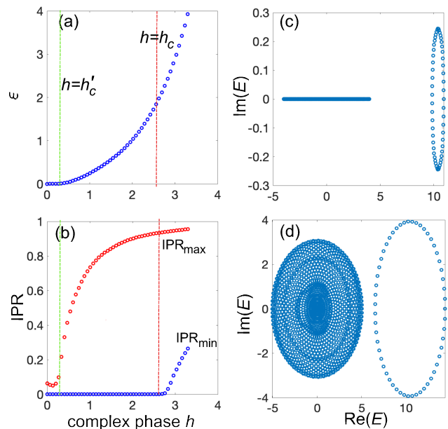
FIG. 5. Same as Fig.3, but for U = 10 .
