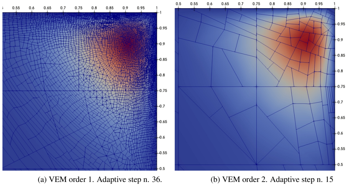
FIG. 7: Test case 1. Zoom of the computed solutions and corresponding anisotropic grids at the final step of the adaptive algorithm based on employing the estimator \eta_h defined in (6.1) to drive the adaptive algorithm.
