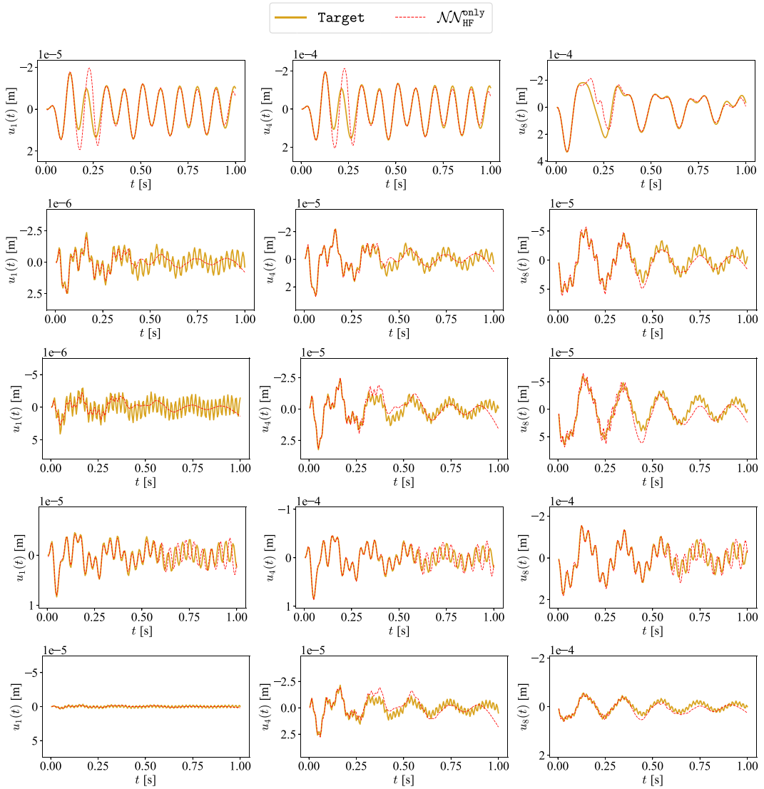
Fig. 8. L-shaped cantilever beam — exemplary comparisons of u_1(t) , u_4(t) and u_8(t) displacement time histories provided by \mathcal{N}_u^{\text{only HF}} with the target HF signals. Results in the five rows are obtained for values of the input parameters taken from the following vectors: Q = \{2.57, 2.61, 4.56, 4.71, 4.90\} kPa; f = \{10.32, 35.10, 46.93, 26.23, 53.26\} Hz; x_d = \{1.70, 3.18, 3.85, 3.85, 3.85\} m; y_d = \{0.15, 0.15, 0.76, 1.28, 1.93\} m.
