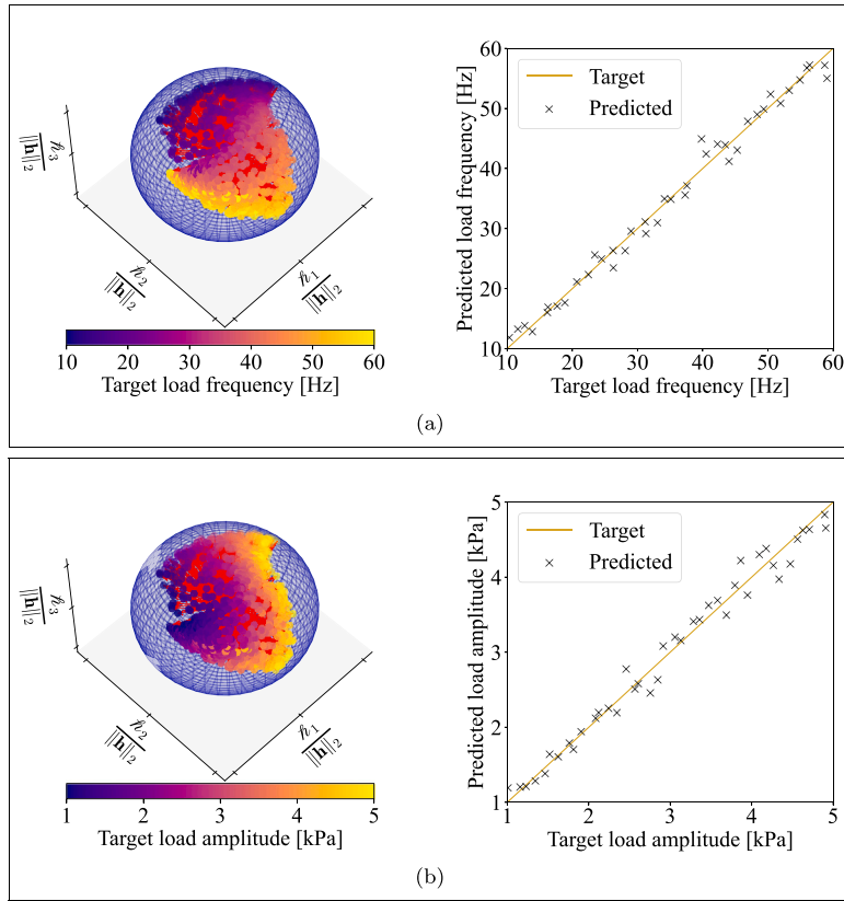
Fig. 15. L-shaped cantilever beam — preliminary identification of the (a) load frequency and (b) load amplitude: (left) normalized embeddings of \mathbf{D}_{\text{HF}} on the unit hypersphere against the target values of the operational conditions; (right) parity plots, relevant to the outcome of the KNN regression over the I_{\text{HF}}^{\text{T}} = 40 noise-contaminated testing instances.
