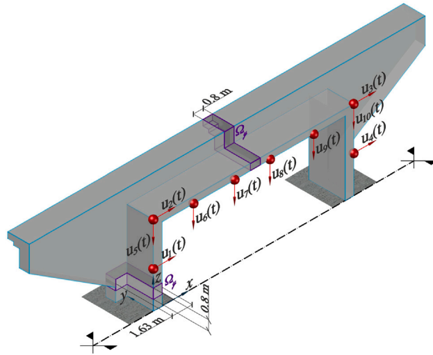
Fig. 10. Railway bridge — physics-based digital twin, perspective cross-section with details of synthetic recordings related to displacements u_1(t), \dots, u_{10}(t) , and damaged region \Omega_d .
