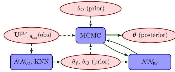
Fig. 13. Flowchart of the online phase of the adopted SHM strategy. Red nodes refer to the input/output quantities, while blue nodes denote the relevant computational blocks: \mathcal{NN}_{OC} and KNN refer to the preliminary (deterministic) identification of the parameters ruling the operational conditions; MCMC refers to the Bayesian inference procedure; \mathcal{NN}_{MF} is the multi-fidelity surrogate model, exploited to systematically speed up the evaluation of the likelihood function while sampling the posterior pdf. (For interpretation of the references to color in this figure legend, the reader is referred to the web version of this article.)
