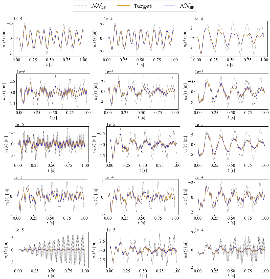
Fig. 7. L-shaped cantilever beam — exemplary comparisons of u_1(t) , u_4(t) and u_8(t) displacement time histories provided by \mathcal{NN}_{LF} and \mathcal{NN}_{HF} with the target HF signals. Results in the five rows are obtained for values of the input parameters taken from the following vectors: Q = \{2.37, 2.61, 4.56, 4.71, 4.90\} kPa; f = \{10.32, 35.10, 46.93, 26.23, 53.26\} Hz; x_D = \{1.70, 3.18, 3.85, 3.85, 3.85\} m; y_D = \{0.15, 0.15, 0.76, 1.28, 1.93\} m.
