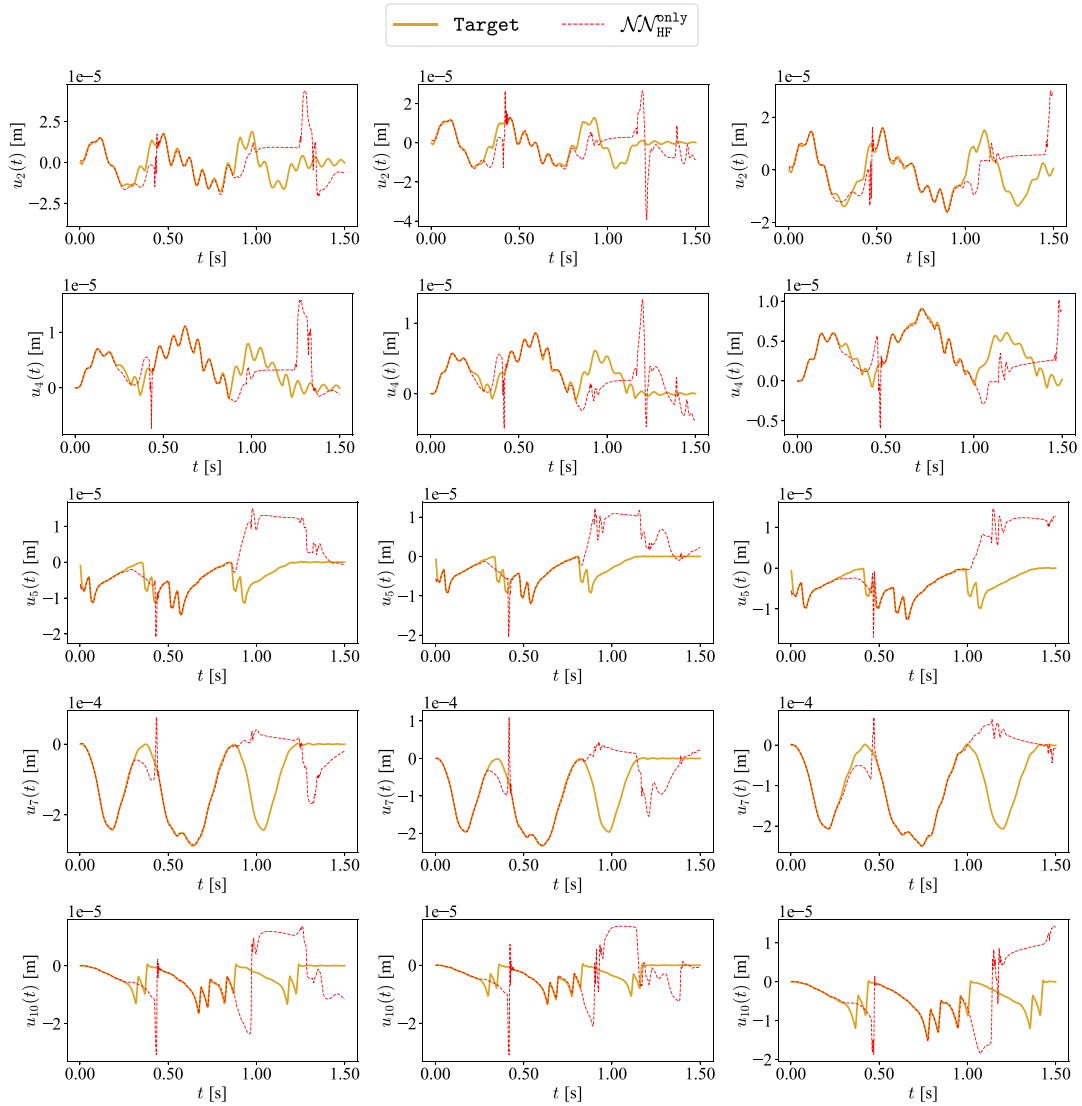
Fig. 12. Railway bridge — exemplary comparisons of u_2(t) , u_4(t) , u_5(t) , u_7(t) and u_{10}(t) displacement time histories provided by \mathcal{N}\mathcal{N}_{HF}^{only} with the target HF signals. Results in the three columns are obtained for values of the input parameters taken from the following vectors: v = \{192.1, 203.48, 166.59\} km/h; \phi = \{20.66, 16.85, 17.95\} ton; x_{\Omega} = \{5.97, 4.95, 16.515\} m; z_{\Omega} = \{6.25, 6.25, 2.46\} m; \delta = \{0.23, 0.42, 0.30\} %.
