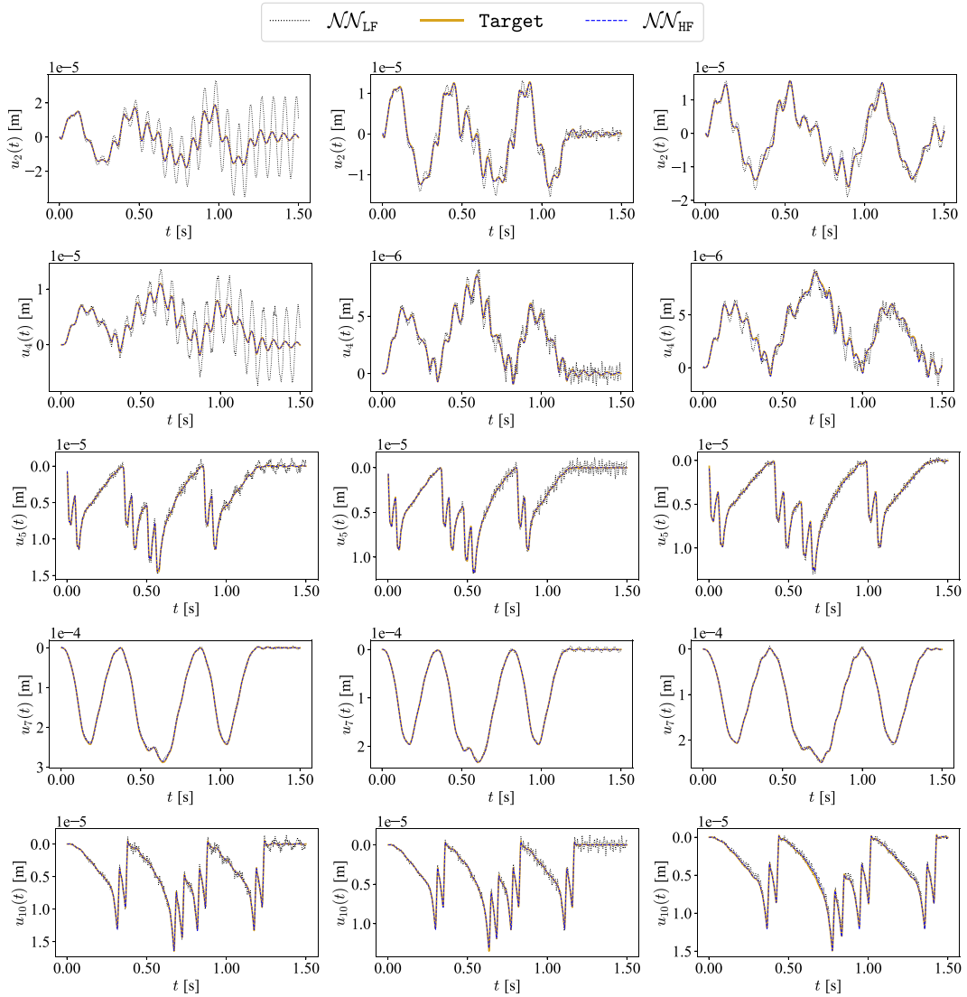
Fig. 11. Railway bridge — exemplary comparisons of u_2(t) , u_4(t) , u_5(t) , u_7(t) and u_{10}(t) displacement time histories provided by \mathcal{NN}_{LF} and \mathcal{NN}_{HF} with the target HF signals. Results in the three columns are obtained for values of the input parameters taken from the following vectors: v = \{192.1, 203.48, 166.59\} km/h; \phi = \{20.66, 16.85, 17.95\} ton; x_{\Omega} = \{5.97, 4.95, 16.515\} m; z_{\Omega} = \{6.25, 6.25, 2.46\} m; \delta = \{0.23, 0.42, 0.30\}\% .
