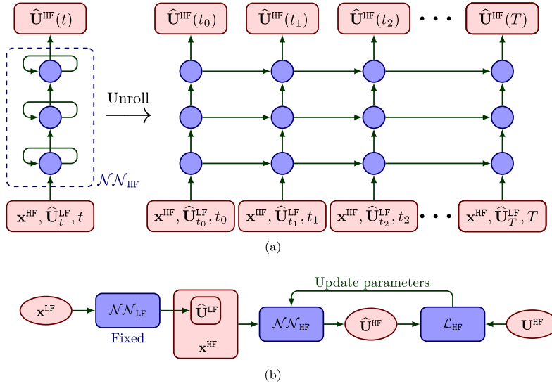
Fig. 4. \mathcal{NN}_{\text{HF}} component: (a) scheme of the recurrent model; (b) training flowchart.
