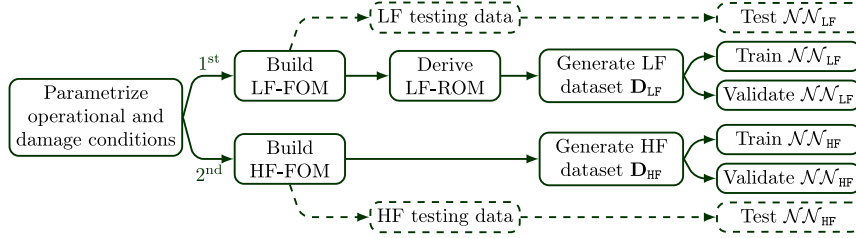
Fig. 5. MF-DNN surrogate modeling: methodology flowchart.
