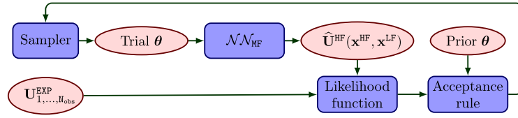
Fig. 16. Scheme of the MCMC procedure to update the probability distribution of the structural state. Red nodes refer to the input/output quantities, while blue nodes denote the relevant computational blocks. (For interpretation of the references to color in this figure legend, the reader is referred to the web version of this article.)
