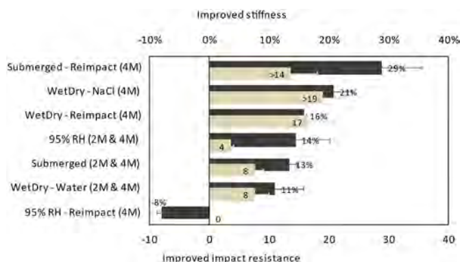
Fig. 15. Stiffness gain (black) and improved impact resistance (grey) of specimens under different healing environments. The difference in deflection between two and four months of healing was not substantial, and results after 2 months were averaged with the ones of four-months specimens in the same healing environment.
