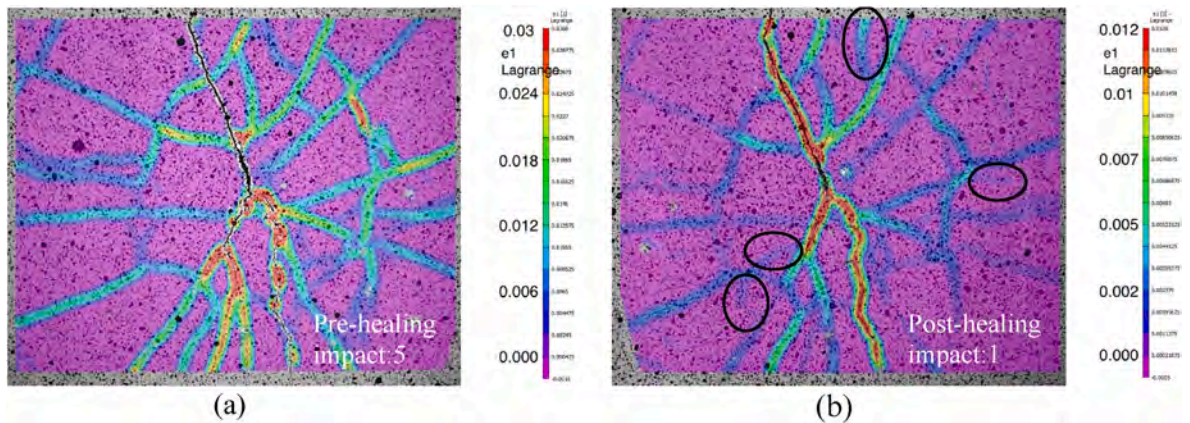
Fig. 11. DIC images of a specimen S3 after five repeated impacts before healing (a) and first impact after healing (b). Black circles in the images indicates the formation of a new crack or a high-strain area.
