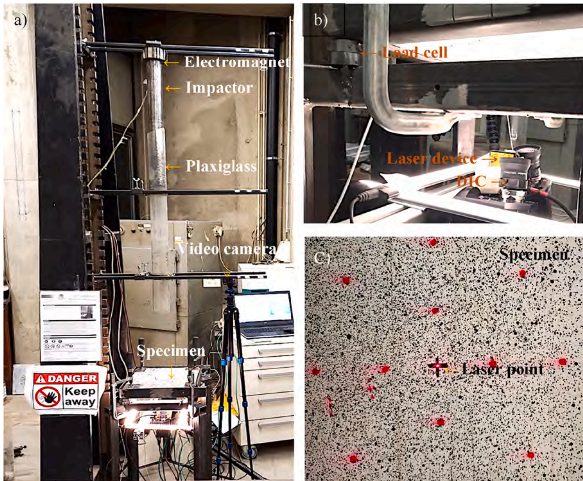
Fig. 2. a) Impact setup with 10 kg impactor released at the height of 1 m above the centre of a specimen, b) Location of DIC, Laser device and load cell, c) Laser pointing at the centre of the specimen.
