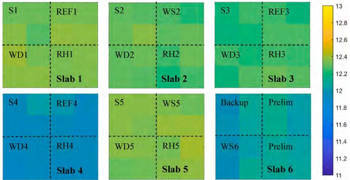
Fig. 1. Slabs steel fibre dispersion charts, colour coded for the measured inductance ( \mu\text{H} ). Slabs were cut into four pieces and allocated to four different healing environments after initial impacts (S: submerged, WD: wet/dry - water, WS: wet/dry - NaCl, RH - 95 \pm 5\% relative humidity).
