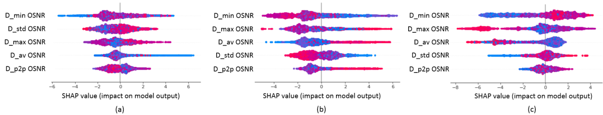
Fig. 3. SHAP summary plot for Single Monitor scenario and fault at (a) link 1, (b) link 2, (c) link 3
