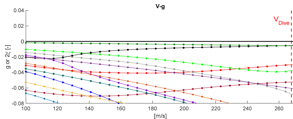
Figure 11. Evolution of the aeroelastic damping vs. TAS for the COMP7 LAM2 \Lambda = 12.24 at corner point altitude z = 8061 m.
