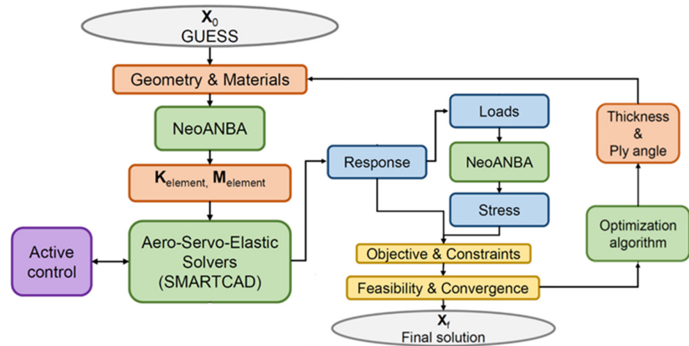
Figure 6. NeOPT's workflow.
