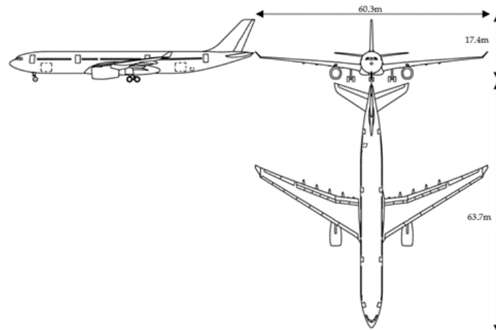
Figure 7. A330-300 tryptic view from [46].
