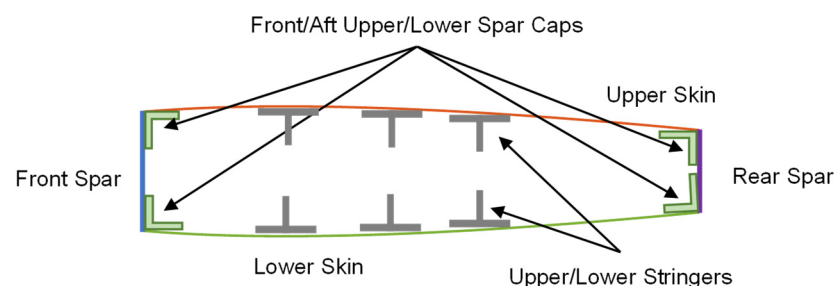
Figure 3. Cross-section components.
