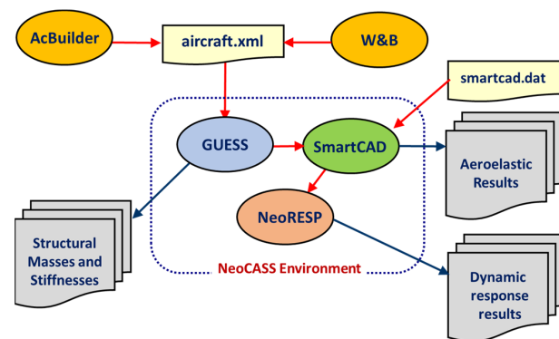
Figure 2. NeoCASS overview.
