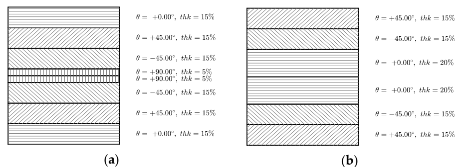
Figure 9. The two stacking sequences used with the percentual thickness (thk) of each ply: (a) LAM1; (b) LAM2.
