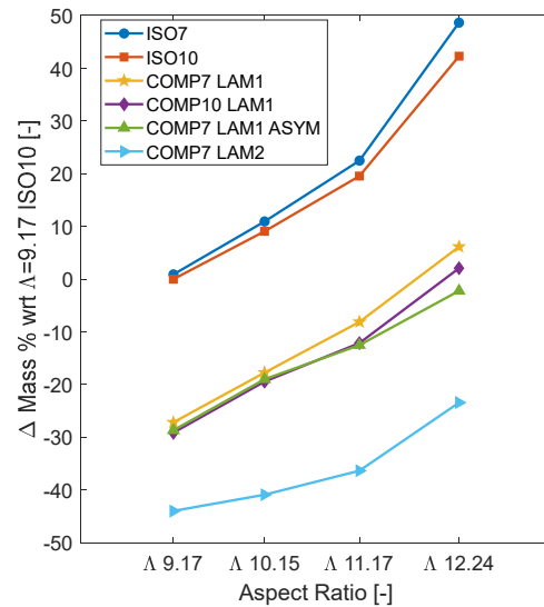
Figure 13. Relative wingbox mass variation with respect to ISO10 \Lambda = 9.17 solution vs. \Lambda .
