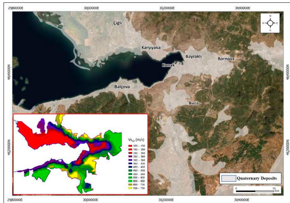
Figure 9. Quaternary deposits map of the metropolitan area of İzmir with the distribution of V_{s30} (average shear wave velocity in the upper 30 m) map. (source: author's elaboration using V_{s30} map obtained from [92] https://temblor.net/earthquake-insights/forensic-analysis-reveals-the-causes-of-building-damage-in-izmir-in-the-oct-30-aegean-sea-earthquake-12098/ (accessed on 20 August 2022). UTM Zone 35S, Datum WGS 84).
