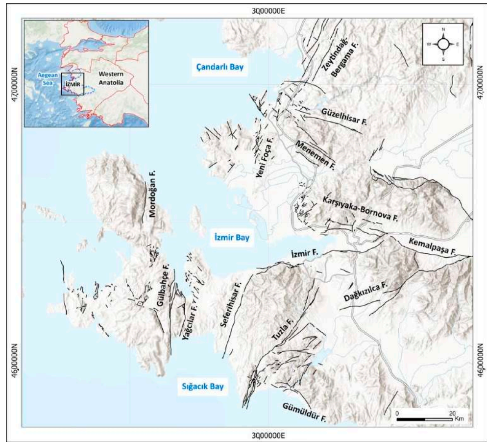
Figure 8. Major fault segments around İzmir. Source: author's elaboration modified after [76] with personal data. UTM Zone 35S, Datum WGS 84).
