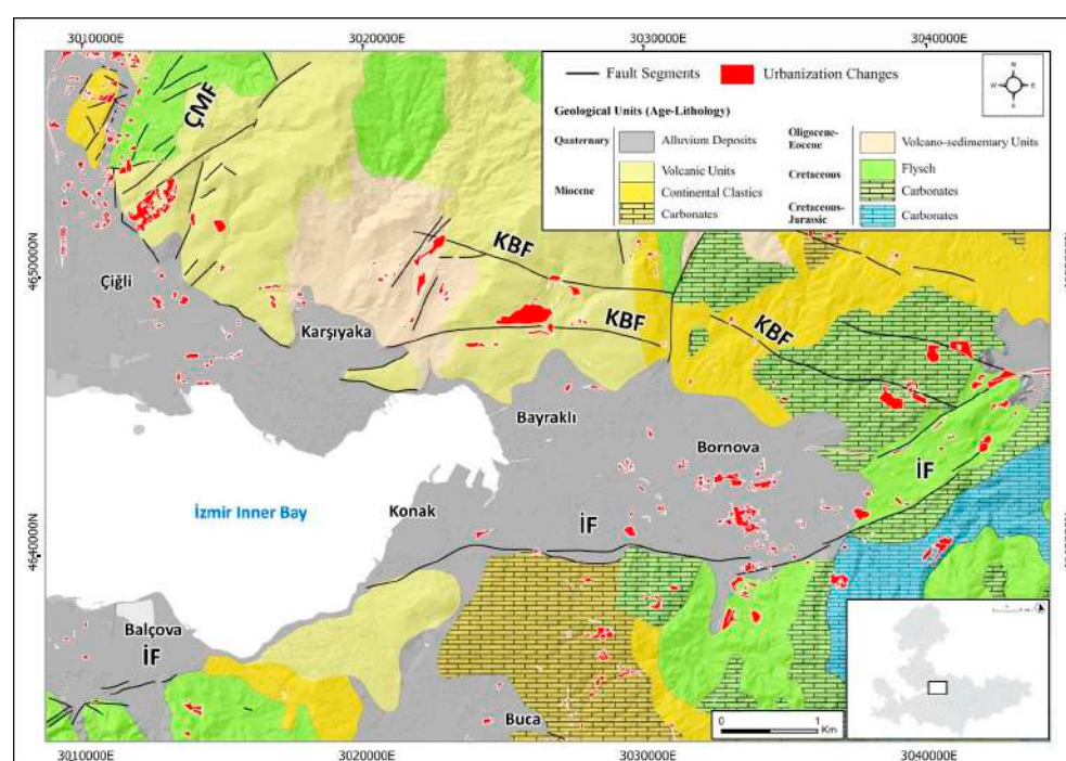
Figure 7. Geological map and urbanization changes in the metropolitan area of İzmir city between 2012 and 2018 (source: author's elaboration modified and digitized from [53,89] and personal data. UTM Zone 35S, Datum WGS 84).
