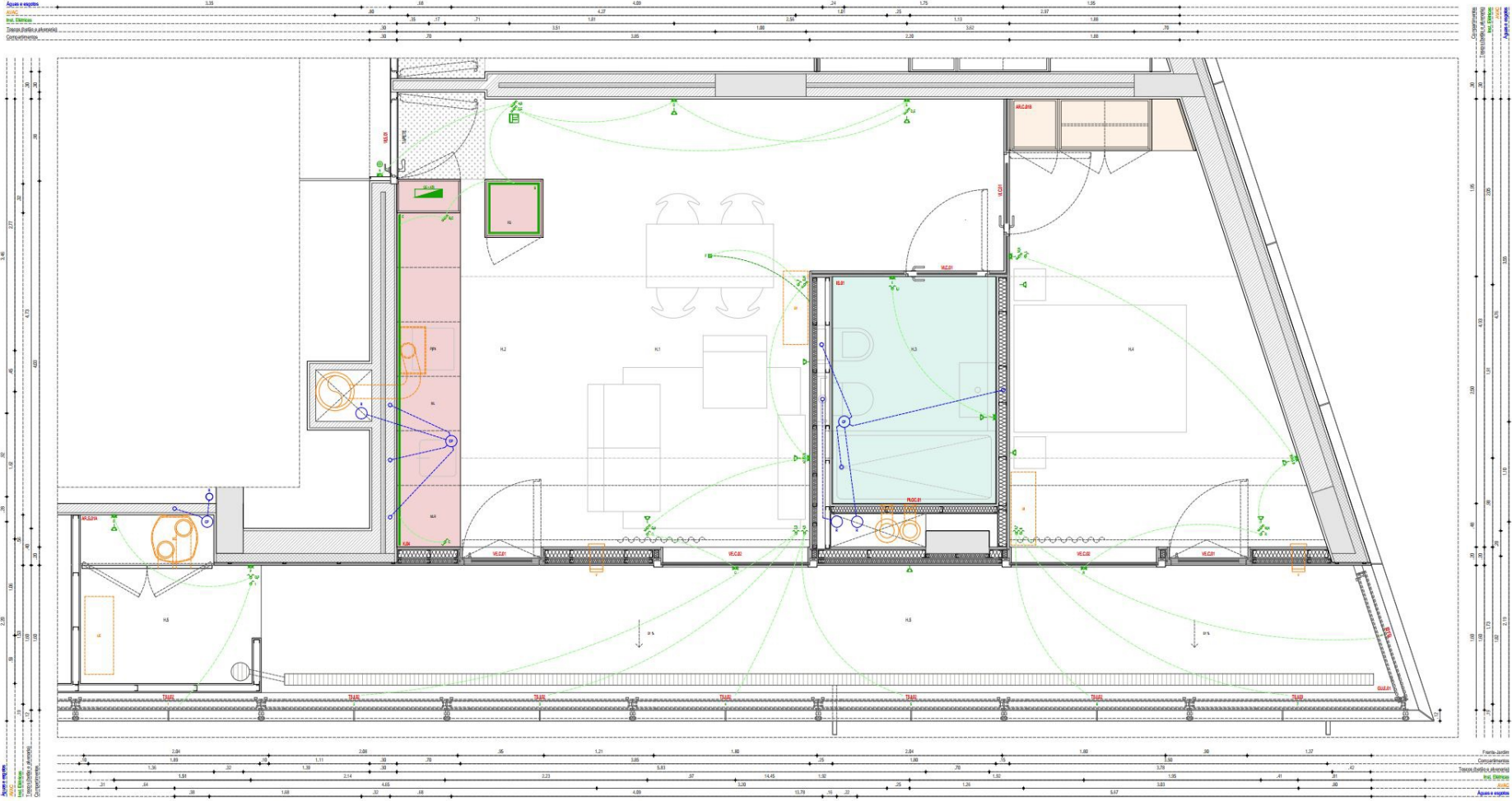
Housing typology – specialties integration
